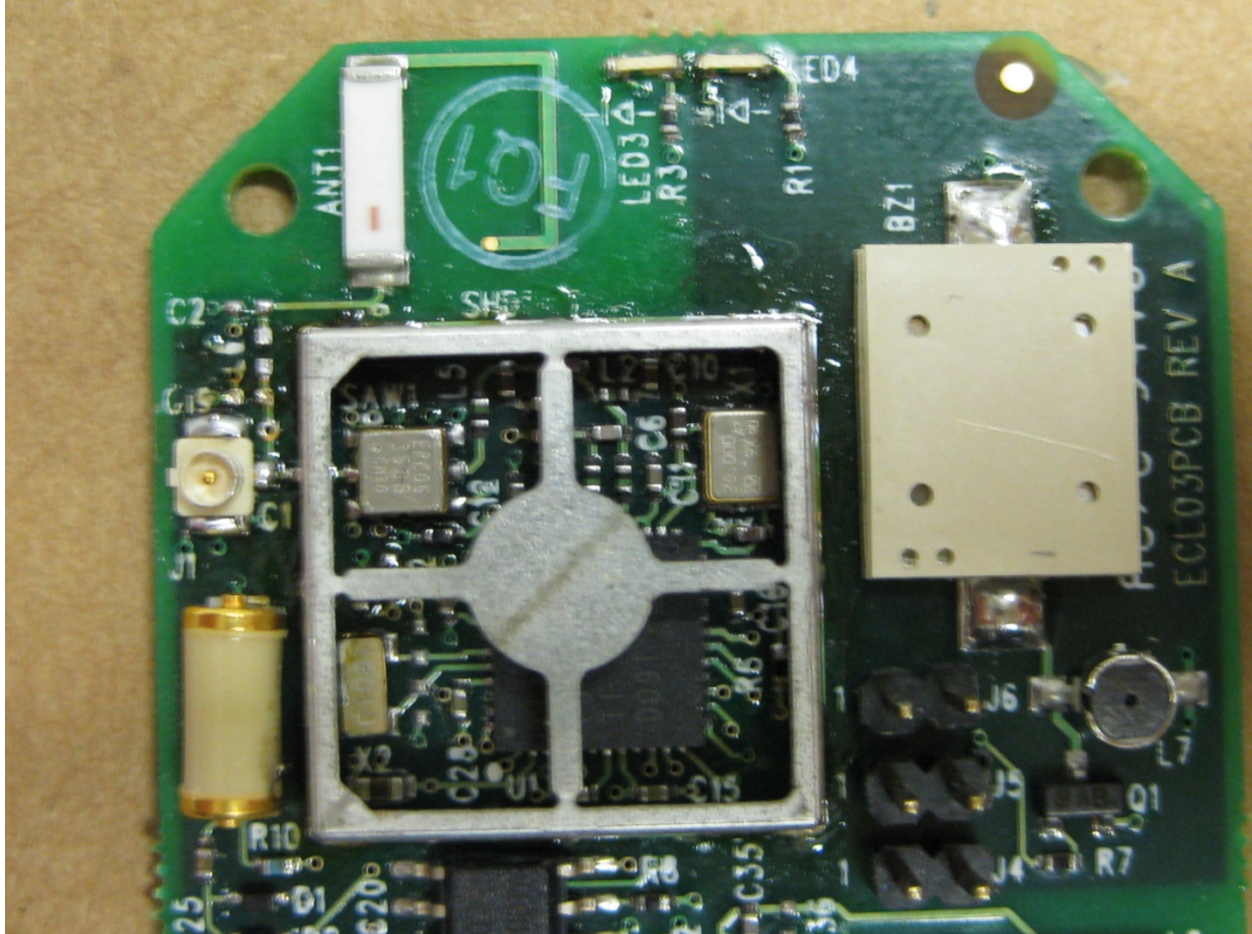
Close-up of RF Section and Chip Antenna
