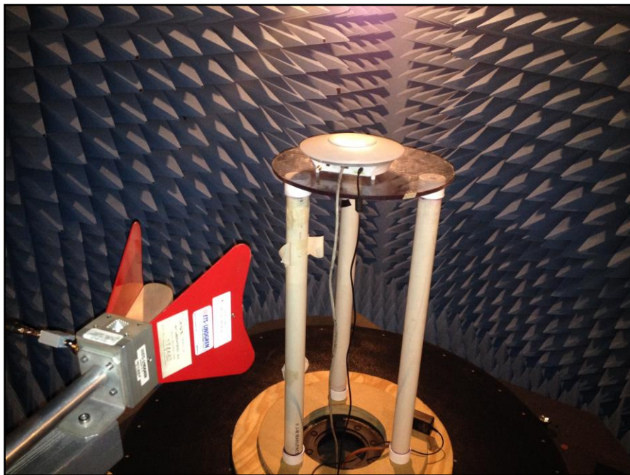
Photograph 7. Radiated Spurs, Test Setup, 1 GHz – 18 GHz, Internal Antenna
