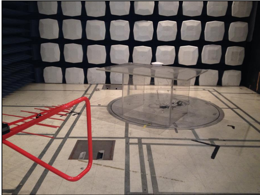
Photograph 6. Radiated Spurs, Test Setup, 30 MHz – 1 GHz, Internal Antenna
