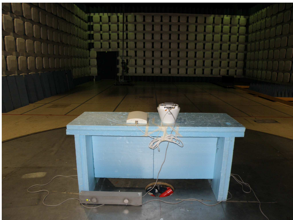
Photograph 2. Radiated emissions measurement
