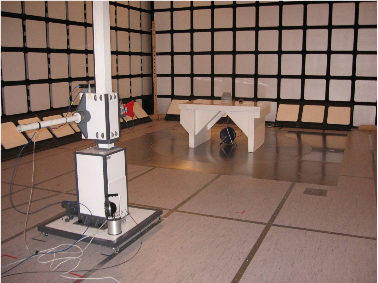
Radiated emissions test setup frequency range 1 – 26 GHz.
