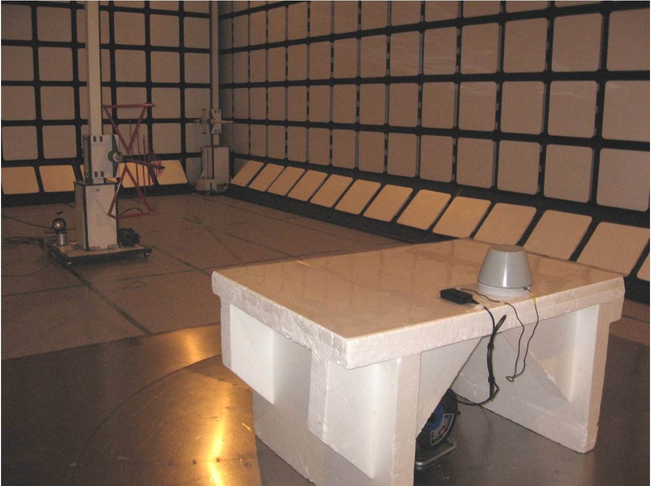
Radiated emissions test setup frequency range 30 – 1000 MHz.
