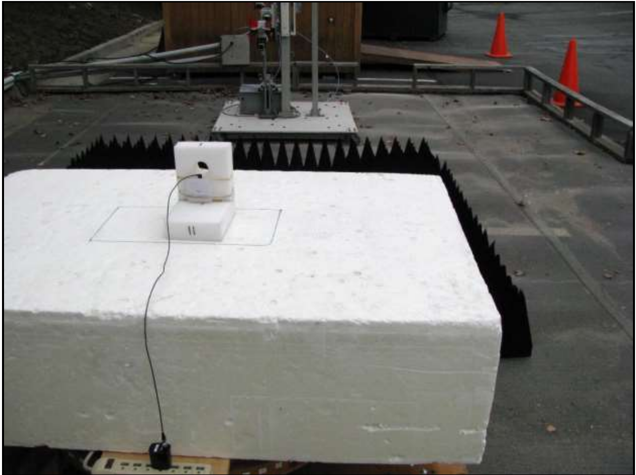
Photograph 4: Radiated Emissions Testing – (Spurious Emissions, >1 GHz)
