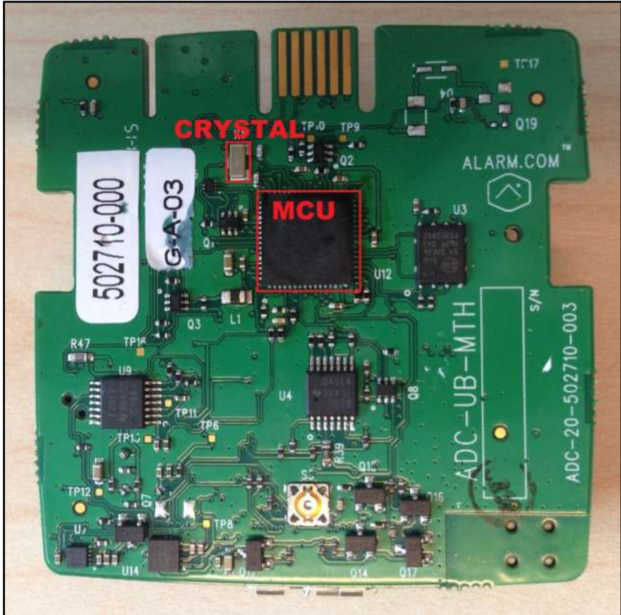
Photograph 17: PCB - Bottom
