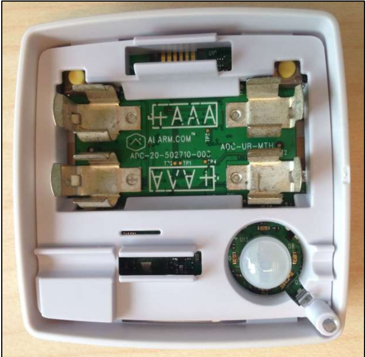
Photograph 15: Inside Casing
