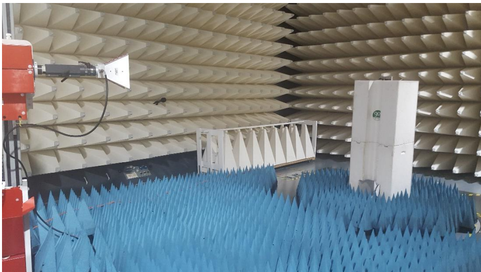
Figure B8. Radiated Setup 2
