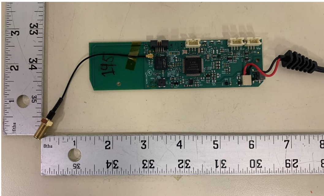
Figure B4. Front view of Conducted DUT
