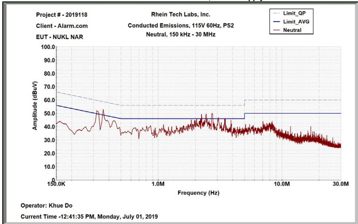
Plot 9-6: Conducted Emissions – Neutral – NA LTE; Power Supply #2
