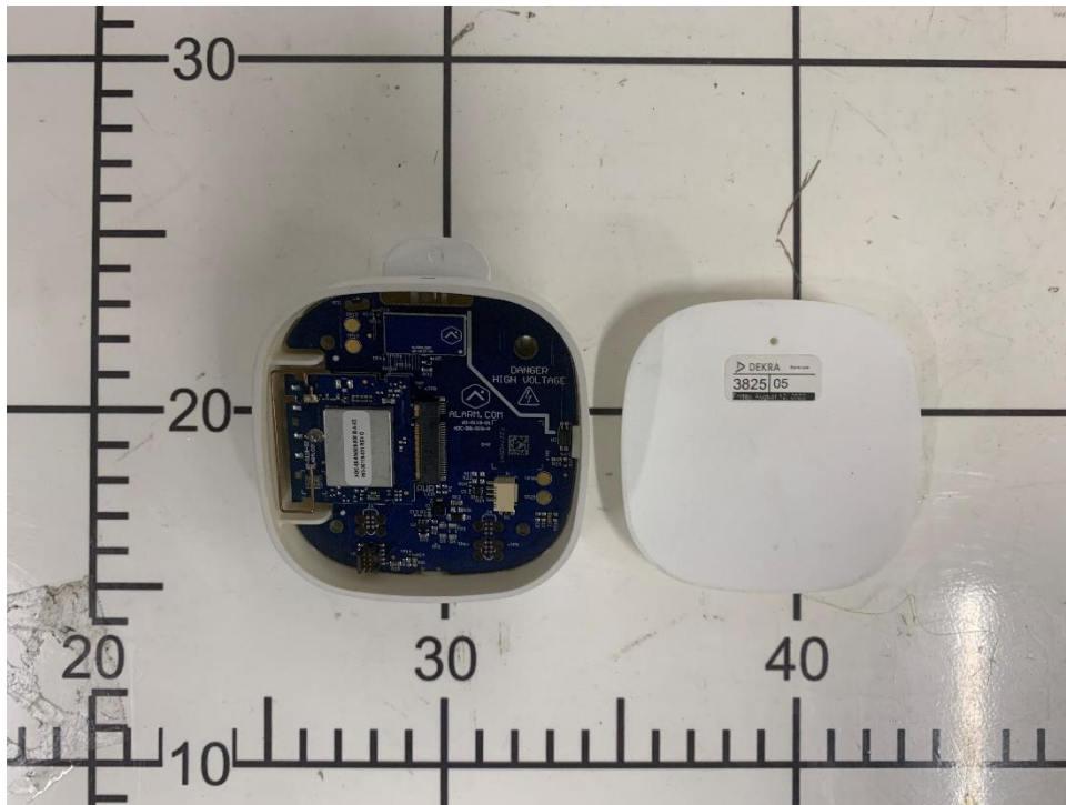
Figure B3. View of the Radiated DUT (Internal)
