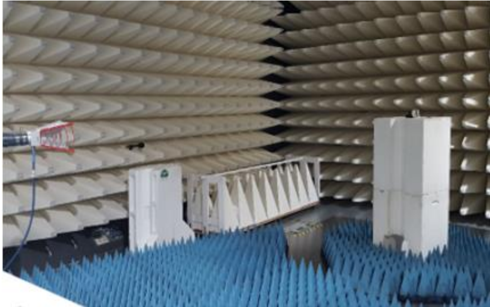
Figure B5. Radiated Test Setup 2
