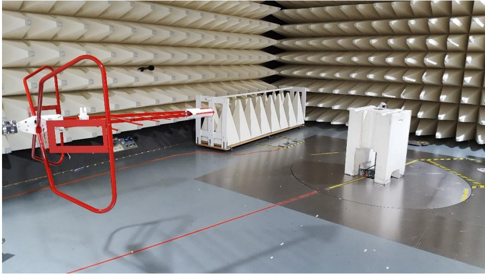
Figure B7. Radiated Setup 1
