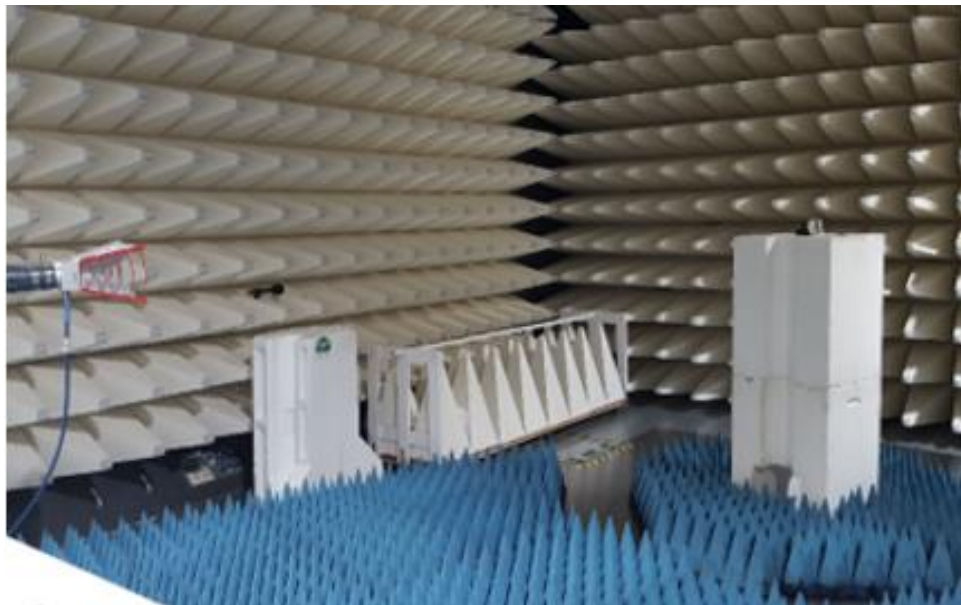
Figure B8. Radiated Setup 2
