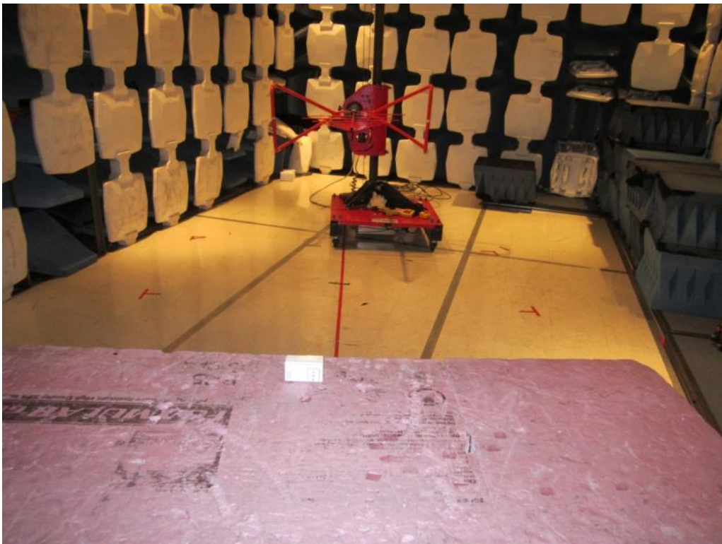
Radiated Emissions – 30 to 1000 MHz (rear)
