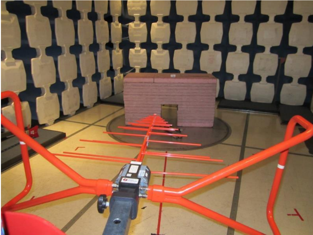
Radiated Emissions – 30 to 1000 MHz (front)
