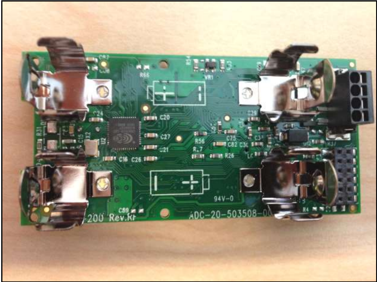
Photograph 7: PCB Side 1
