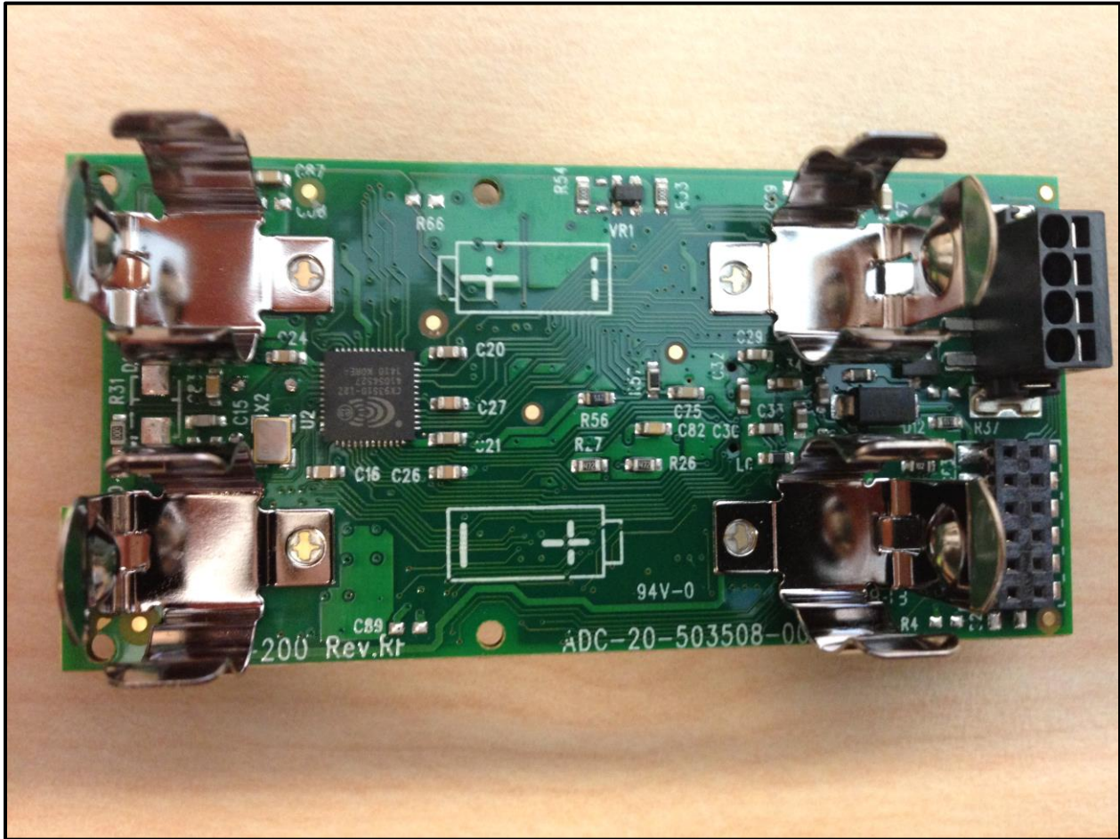
Photograph 6: PCB Side 1
