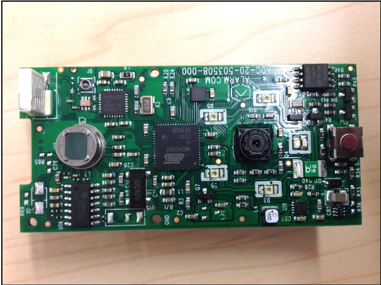
Photograph 7: PCB Side 2
