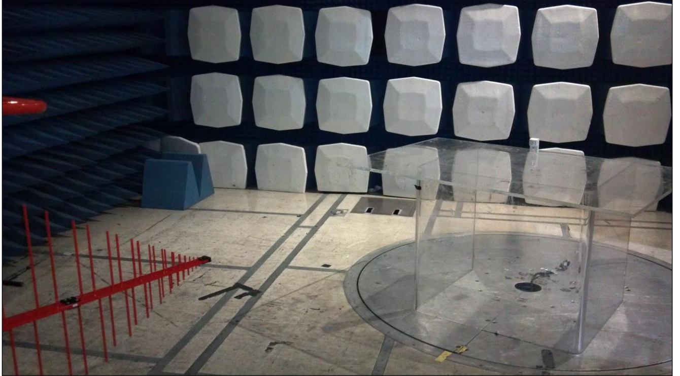
Photograph 1. Radiated Emissions, Test Setup
