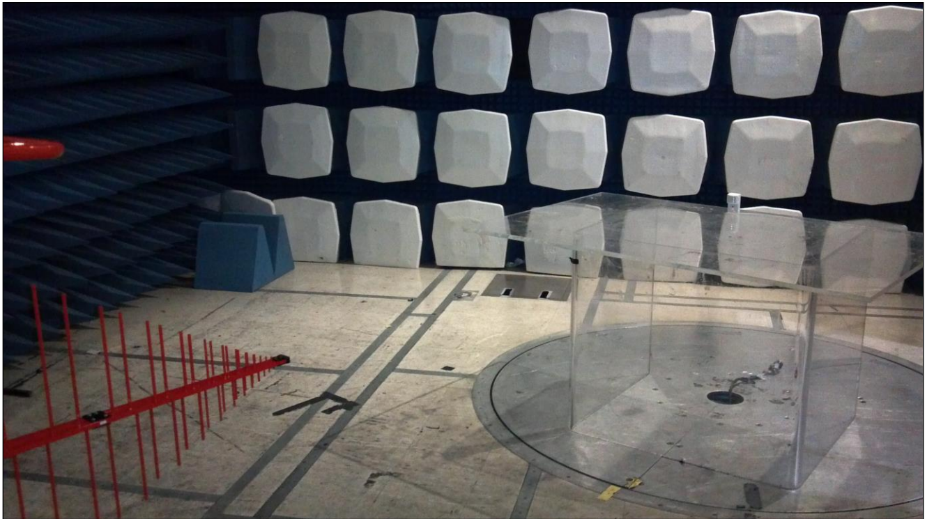
Photograph 2. Radiated Spurious Emissions, Test Setup
