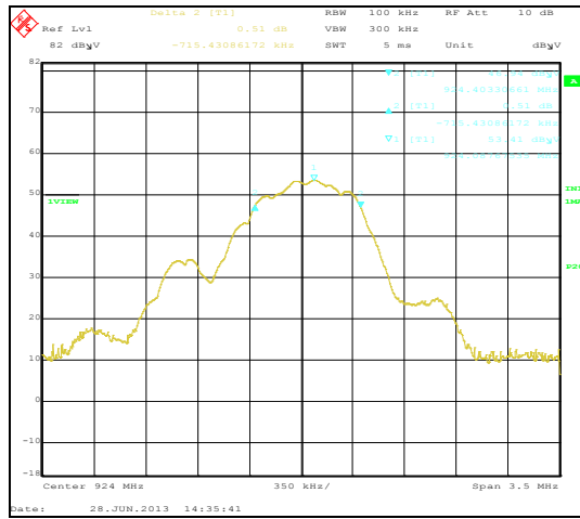
Plot 3. 6 dB Occupied Bandwidth, Low Channel
