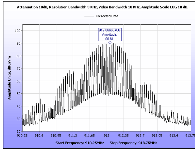
Plot 32. Peak Power Spectral Density, Low Channel
