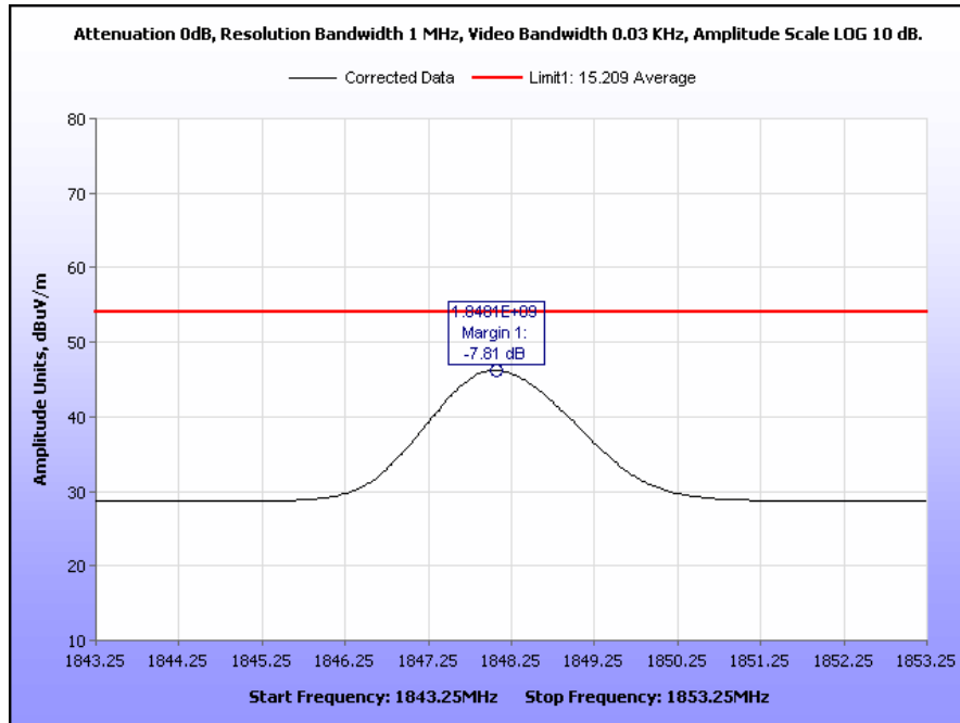
Plot 30. Radiated Spurious Emissions, §15.209, 1800 MHz, High Channel
