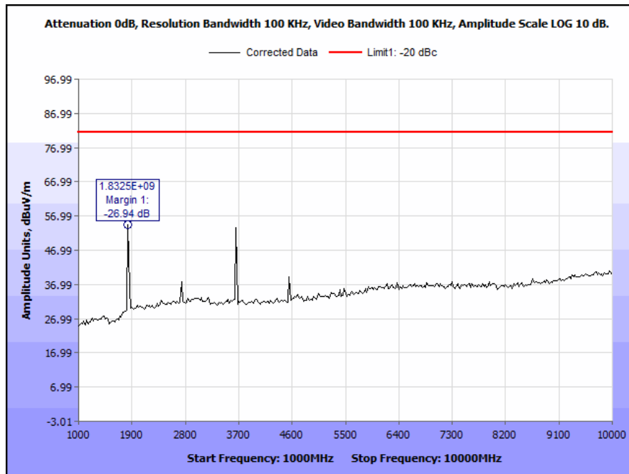
Plot 13. Radiated Spurious Emissions, Low Channel, 1 GHz – 10 GHz, 100 kHz
