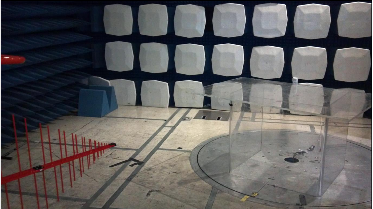
Photograph 3. Radiated Emissions, Test Setup
