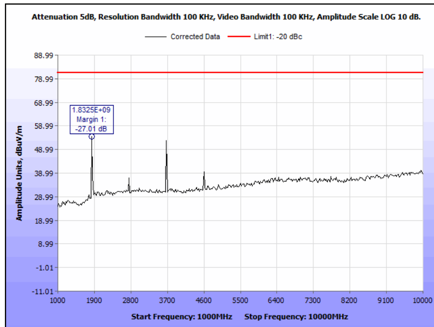
Plot 15. Radiated Spurious Emissions, Mid Channel, 1 GHz – 10 GHz, 100 kHz
