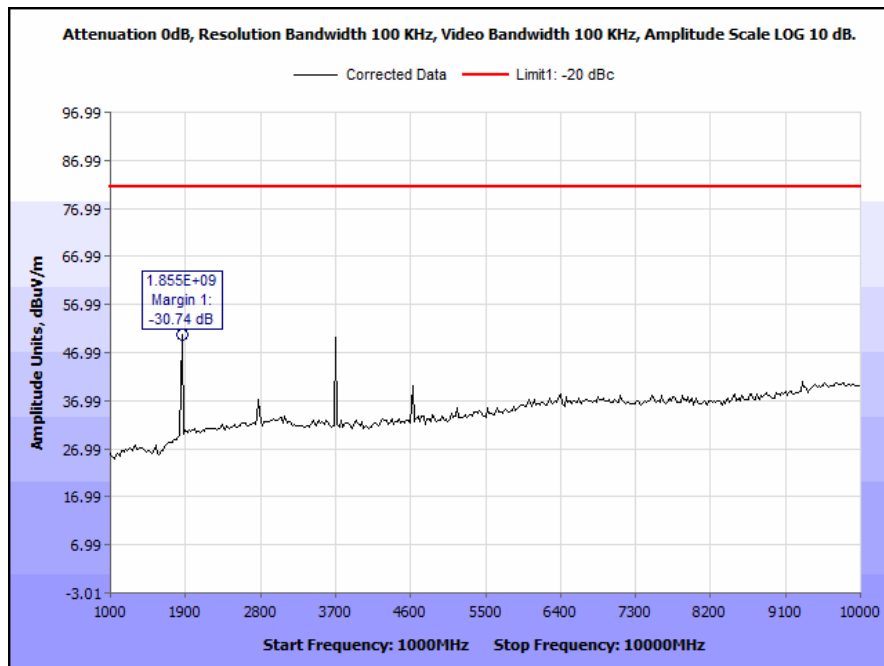
Plot 17. Radiated Spurious Emissions, High Channel, 1 GHz – 10 GHz, 100 kHz
