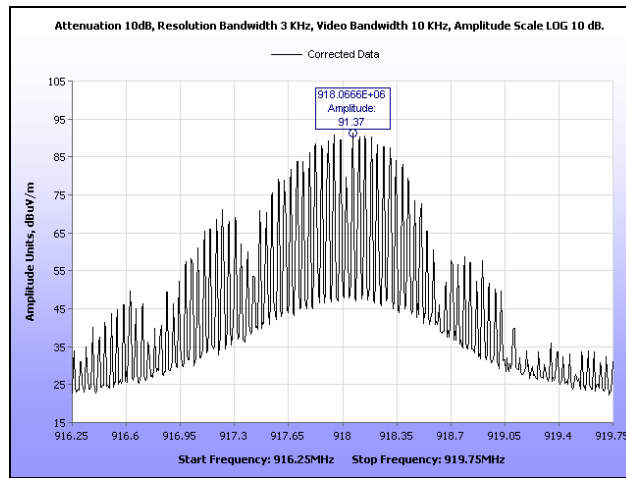
Plot 33. Peak Power Spectral Density, Mid Channel
