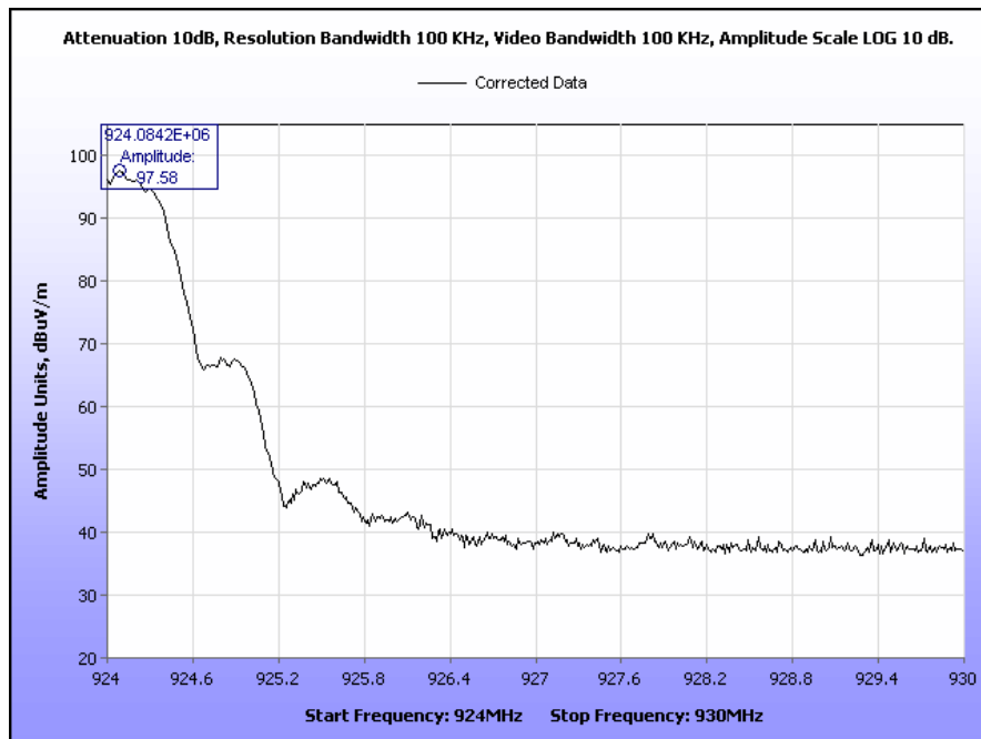
Plot 19. Radiated Spurious Emissions, Band Edge, High Channel
