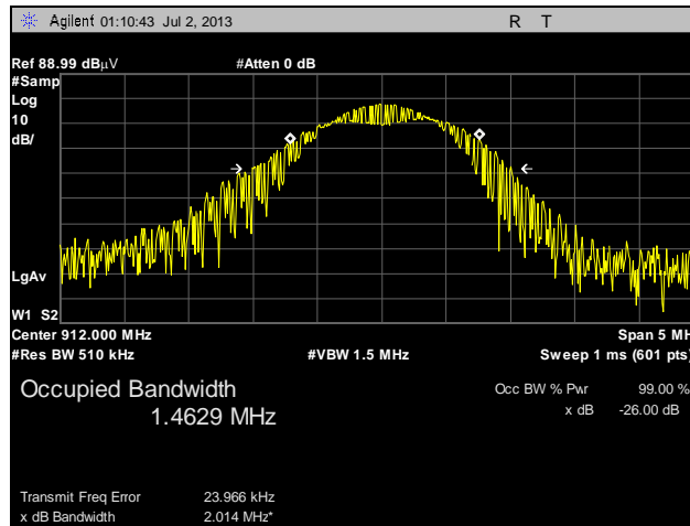
Plot 6. 99% Occupied Bandwidth, Low Channel
