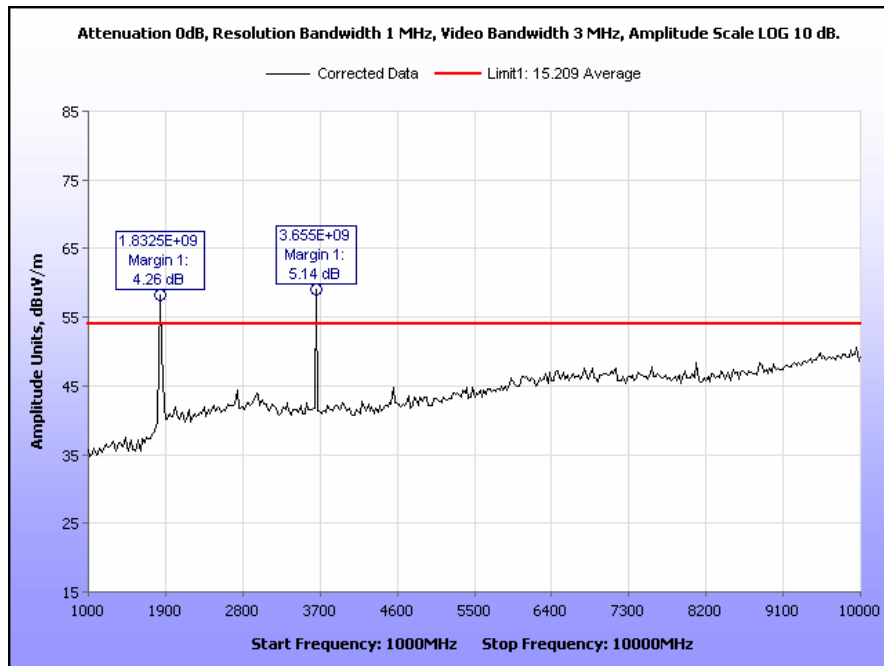
Plot 21. Radiated Spurious Emissions, §15.209, 1 GHz – 10 GHz, Low Channel, Peak Under Average
