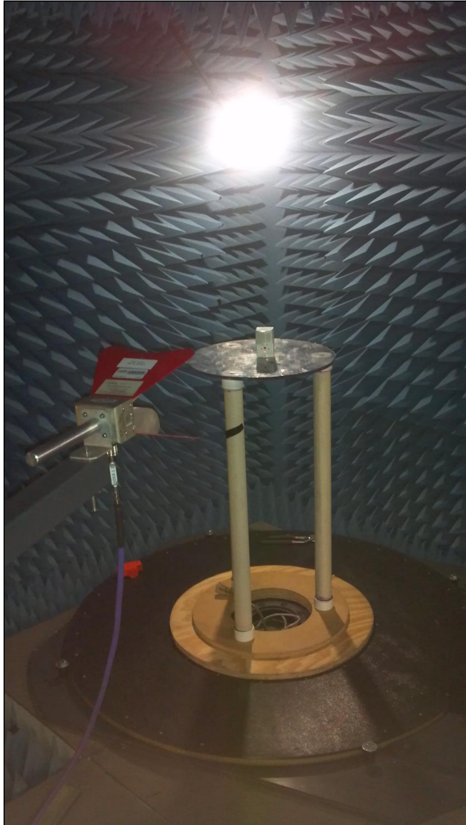
Photograph 5. Radiated Spurious Emissions, 1 GHz to 10 GHz, Test Setup
