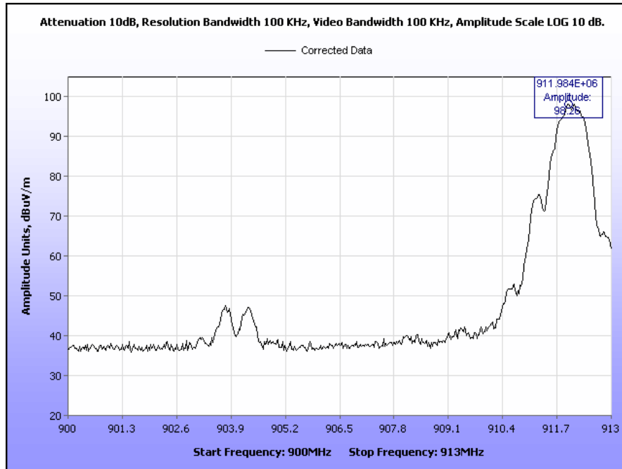
Plot 18. Radiated Spurious Emissions, Band Edge, Low Channel
