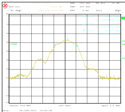
Plot 4. 6 dB Occupied Bandwidth, Mid Channel
