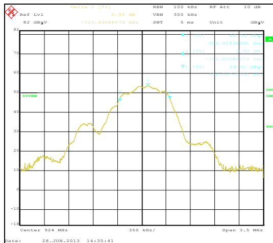
Plot 5. 6 dB Occupied Bandwidth, High Channel
