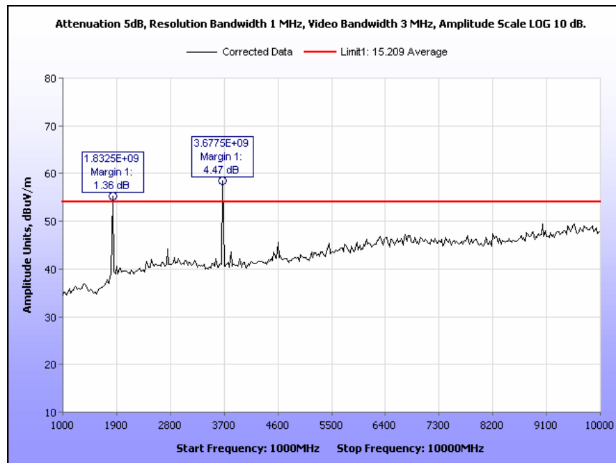
Plot 25. Radiated Spurious Emissions, §15.209, 1 GHz – 10 GHz, Mid Channel, Peak Under Average
