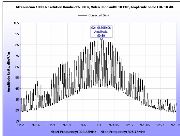
Plot 34. Peak Power Spectral Density, High Channel
