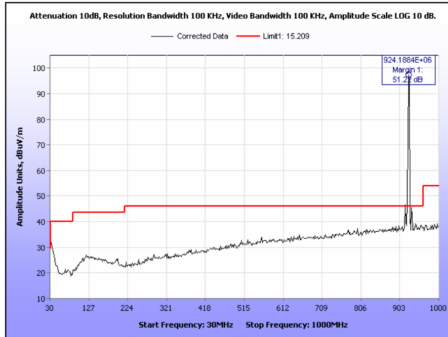
Plot 28. Radiated Spurious Emissions, §15.209, 30 MHz – 1 GHz, High Channel
