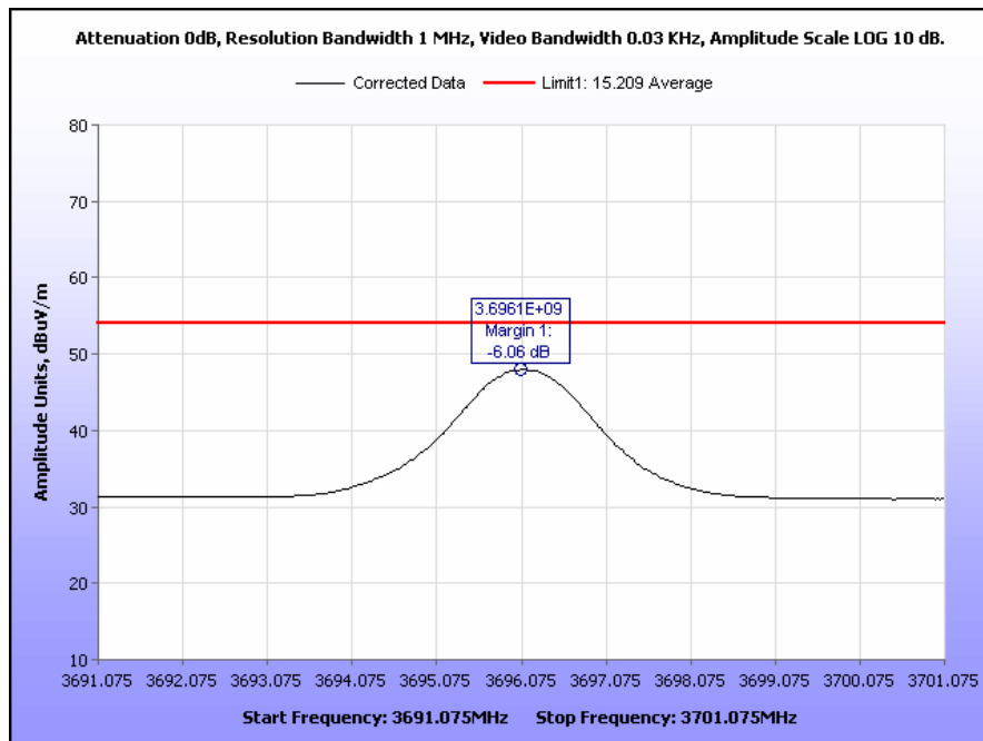
Plot 31. Radiated Spurious Emissions, §15.209, 3700 MHz, High Channel
