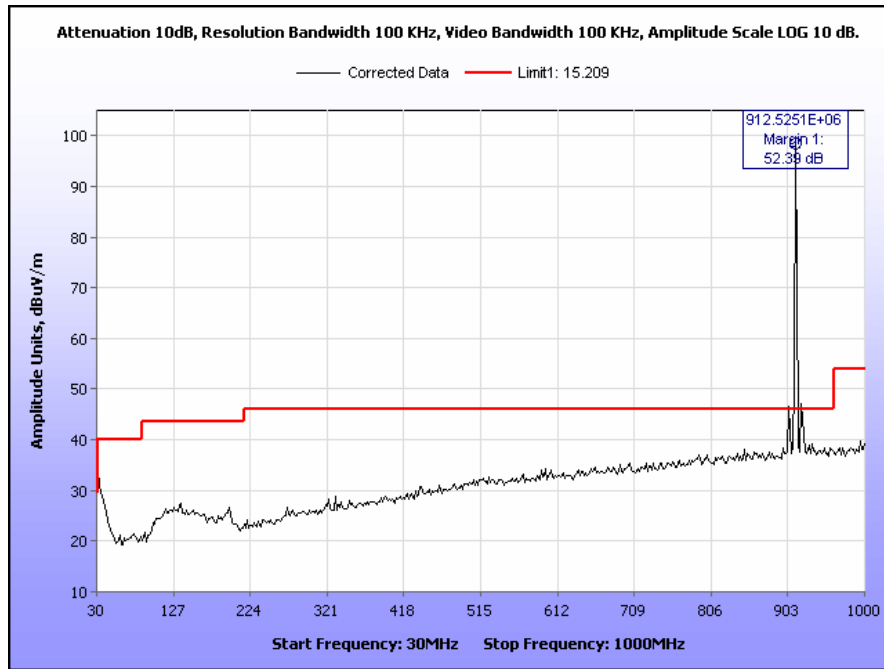
Plot 20. Radiated Spurious Emissions, §15.209, 30 MHz – 1 GHz, Low Channel
