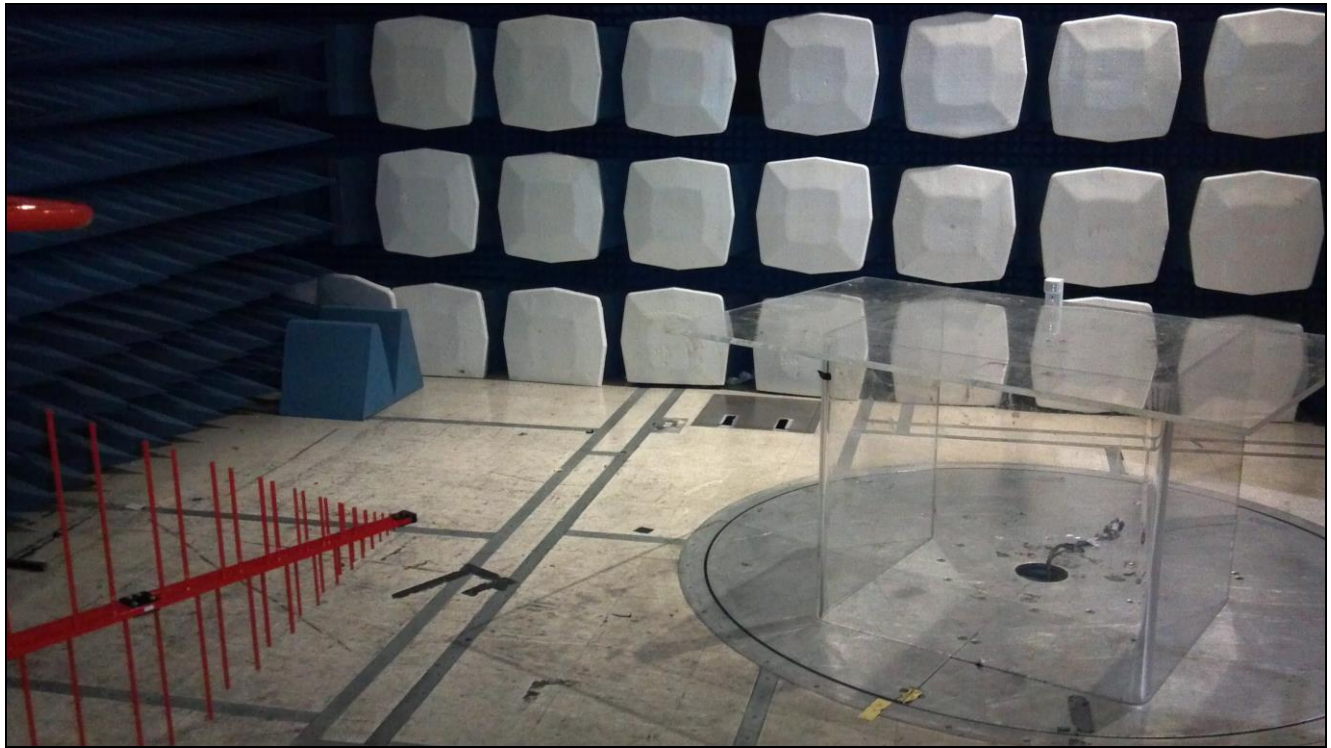
Photograph 4. Radiated Spurious Emissions, 30 MHz to 1 GHz, Test Setup
