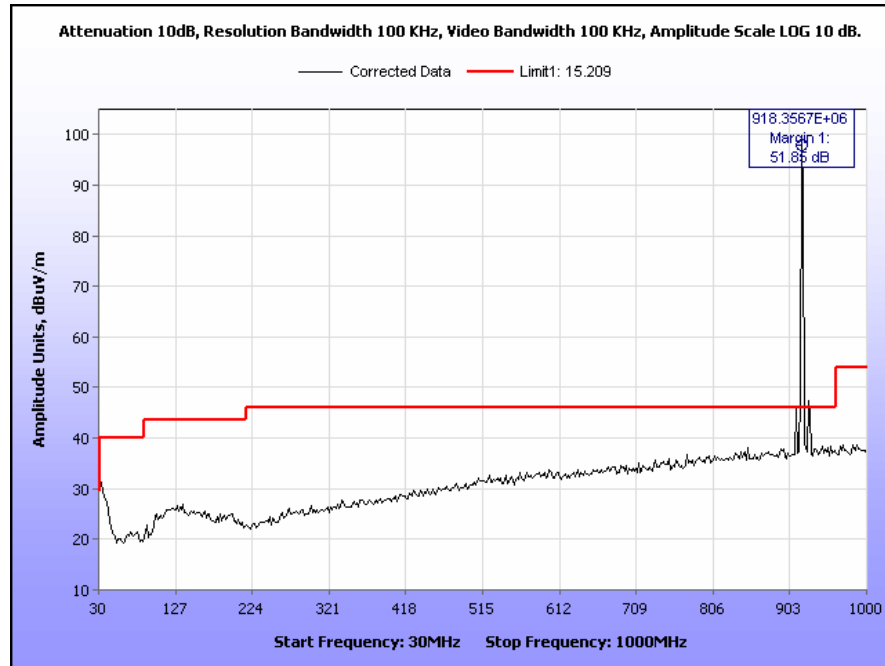
Plot 24. Radiated Spurious Emissions, §15.209, 30 MHz – 1 GHz, Mid Channel
