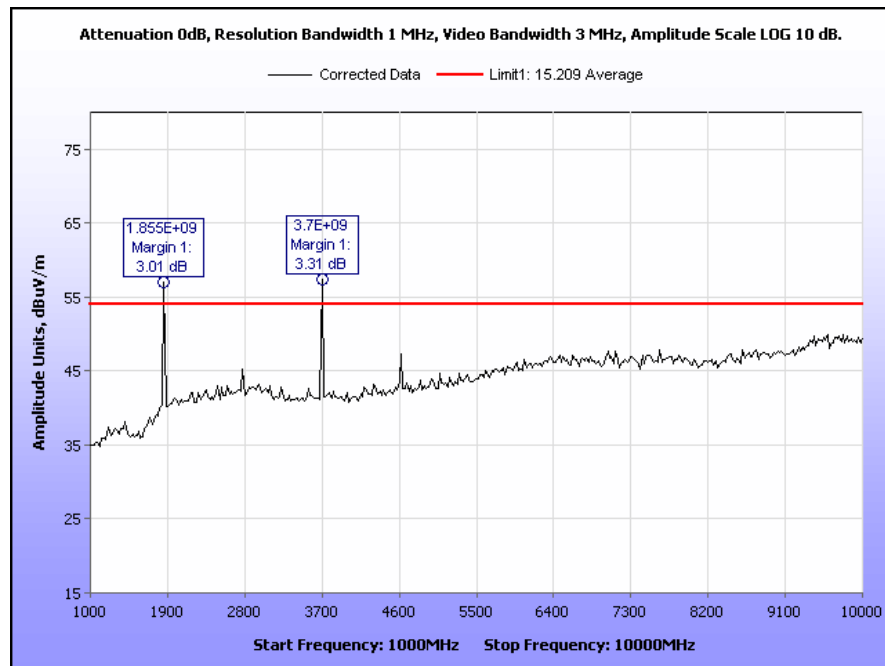
Plot 29. Radiated Spurious Emissions, §15.209, 1 GHz – 10 GHz, High Channel, Peak Under Average
