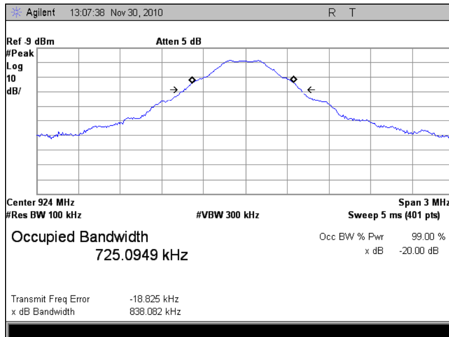
Plot 8. Occupied Bandwidth, High Channel FCC Limits
