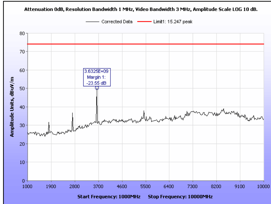
Plot 13. Radiated Spurious Emissions, Low Channel, Peak
