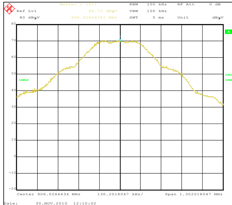
Plot 3. Fundamental Field Strength, Low Channel, Peak Detector
