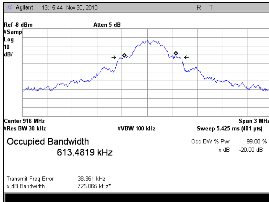
Plot 10. Occupied Bandwidth, Mid Channel, IC Limits
