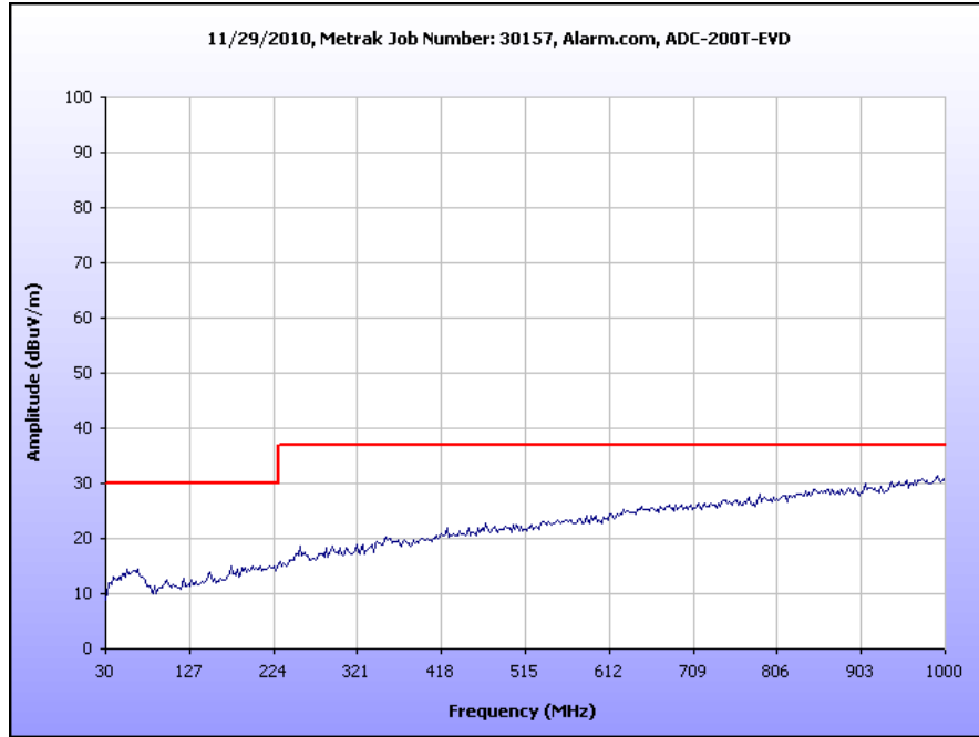
Plot 23. Receiver Spurious Emission, 30 MHz – 1 GHz
