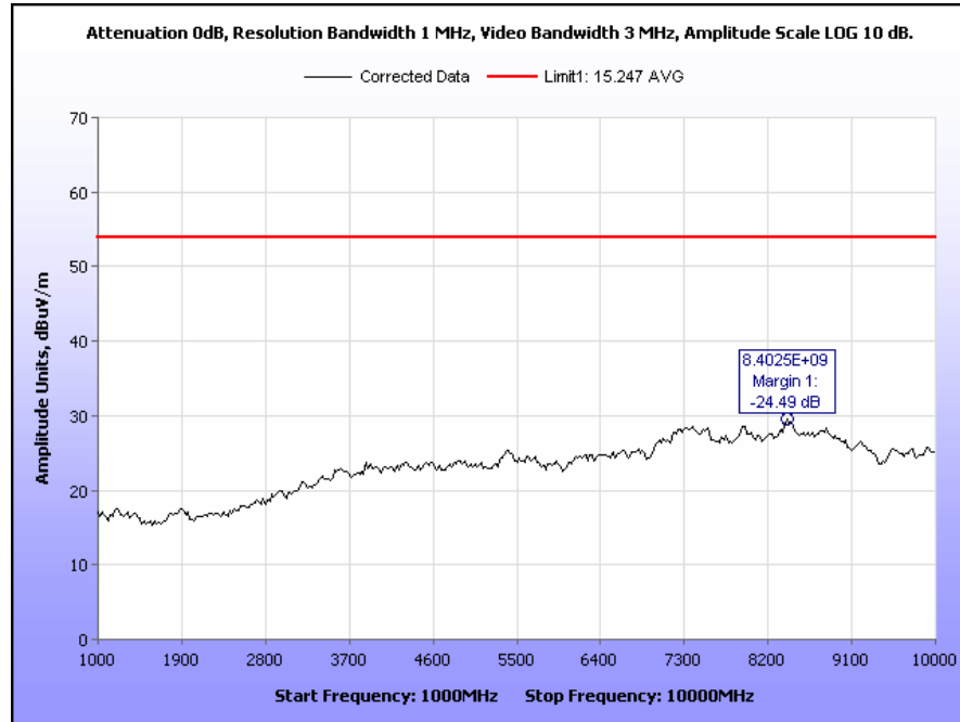
Plot 25. Receiver Spurious Emission, 1 GHz – 10 GHz, Average
