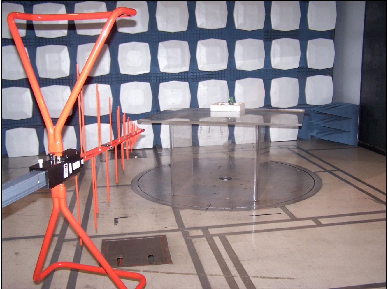
Photograph 3. Transceiver Spurious Emissions, Test Setup
