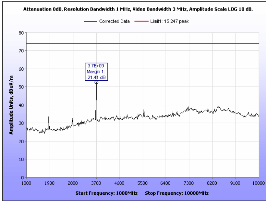
Plot 19. Radiated Spurious Emissions, High Channel, Peak
