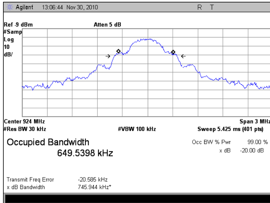
Plot 11. Occupied Bandwidth, High Channel, IC Limits
