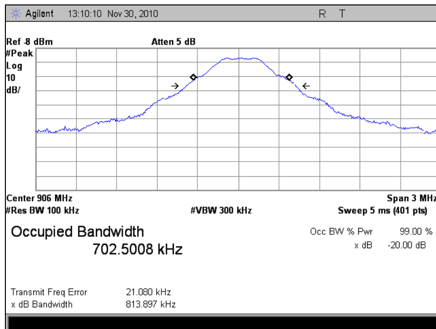
Plot 6. Occupied Bandwidth, Low Channel FCC Limits
