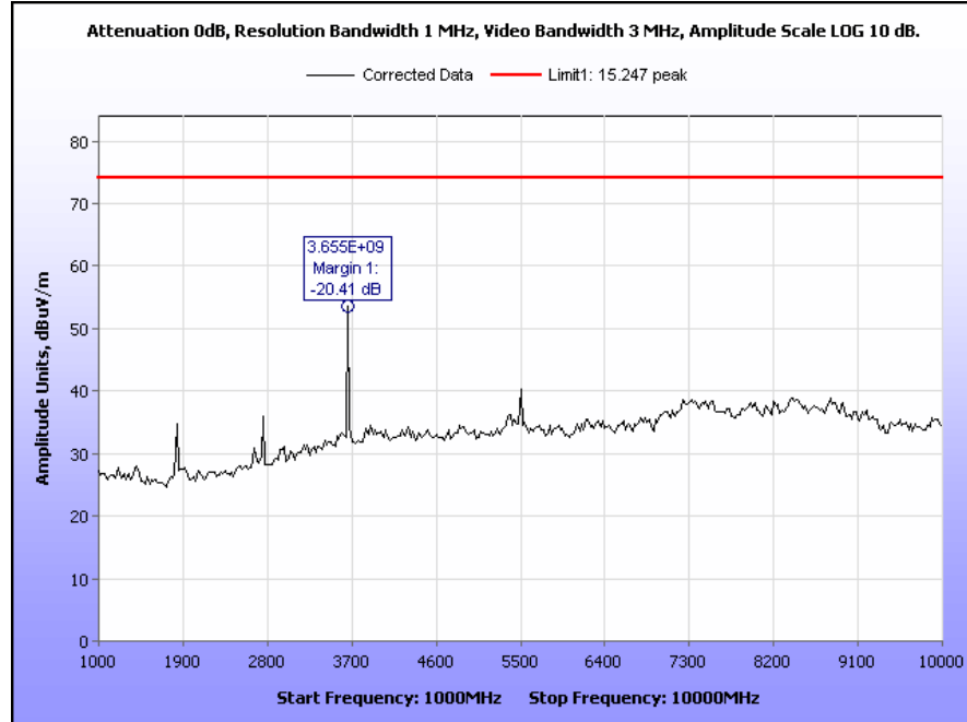
Plot 16. Radiated Spurious Emissions, Mid Channel, Peak
