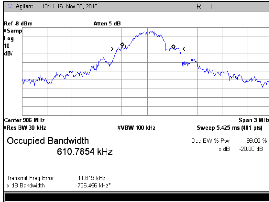
Plot 9. Occupied Bandwidth, Low Channel, IC Limits
