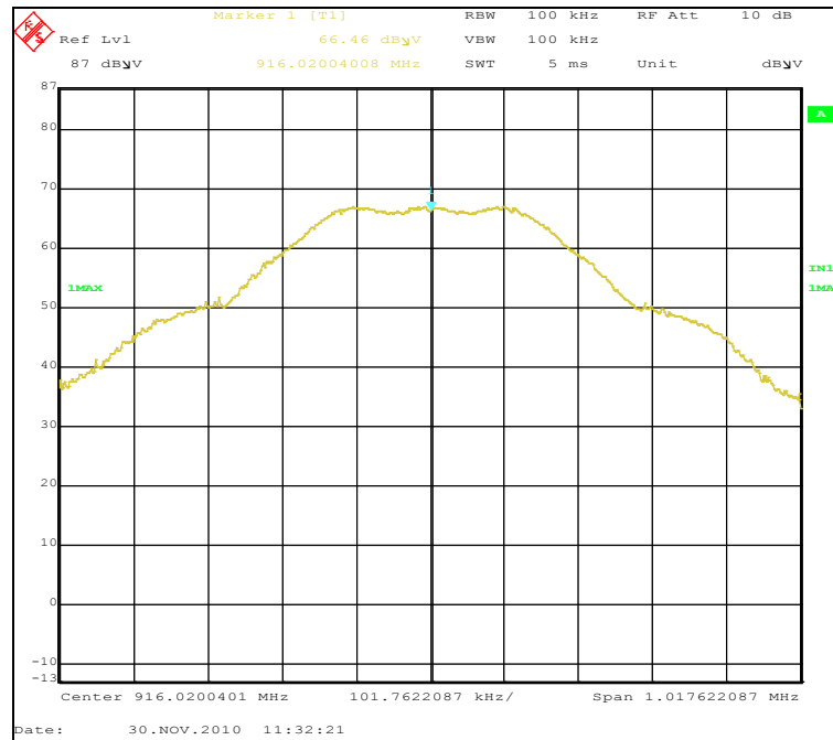
Plot 4. Fundamental Field Strength, Mid Channel, Peak Detector
