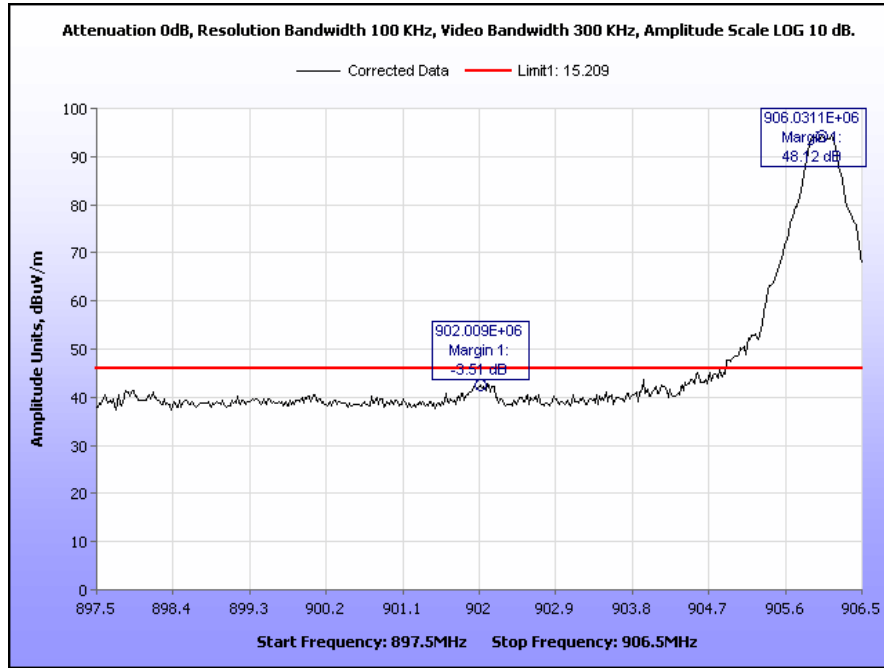
Plot 21. Band Edge, Low Channel
