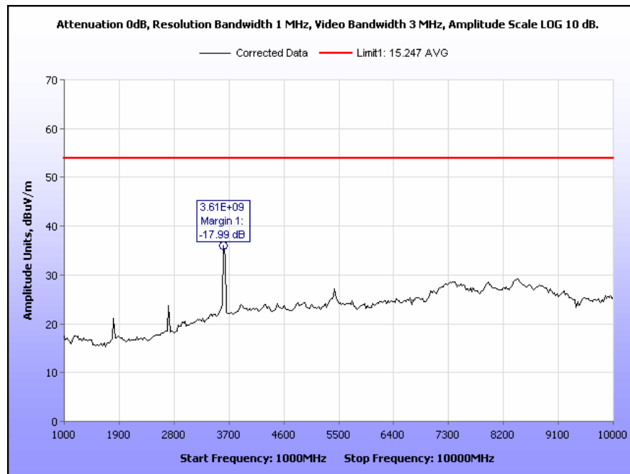
Plot 14. Radiated Spurious Emissions, Low Channel, Average
