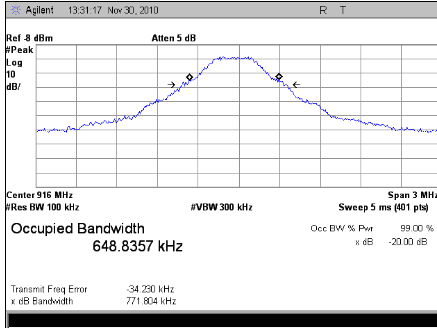
Plot 7. Occupied Bandwidth, Mid Channel FCC Limits
