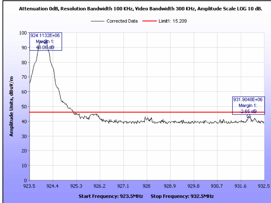
Plot 22. Band Edge, High Channel
