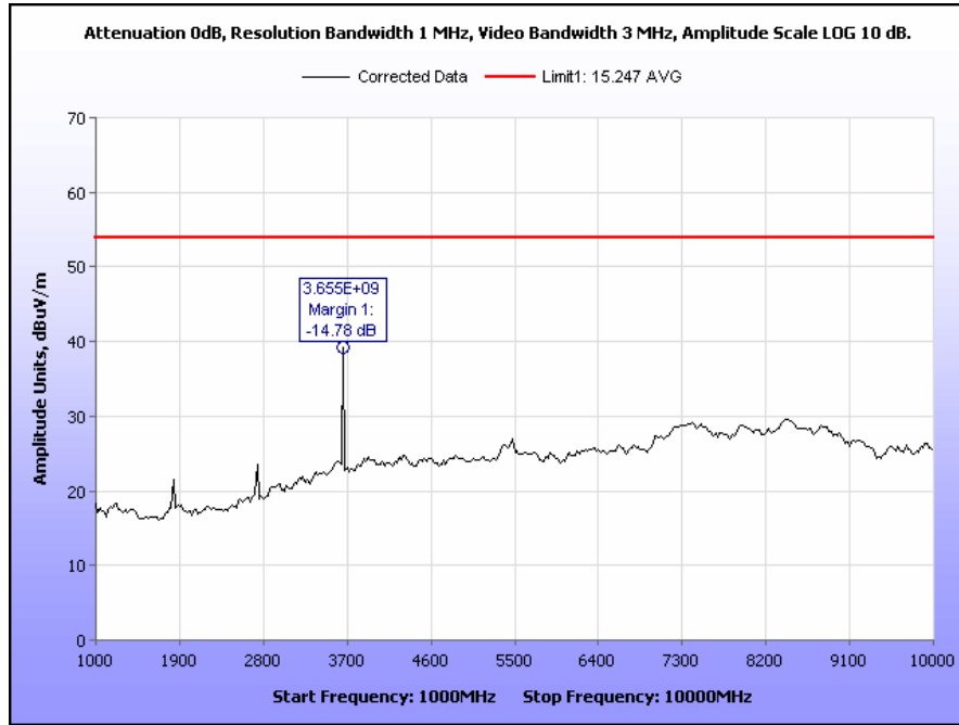
Plot 17. Radiated Spurious Emissions, Mid Channel, Average
