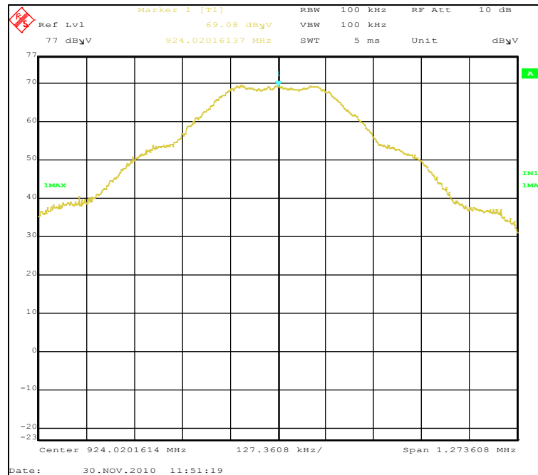
Plot 5. Fundamental Field Strength, High Channel, Peak Detector
