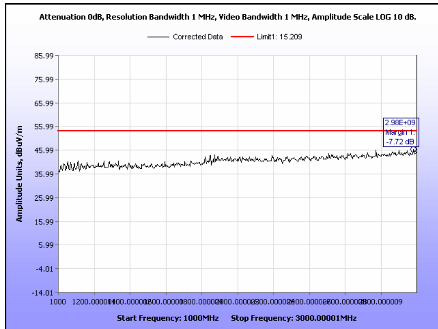
Plot 24. Transmitter Spurious Emissions, High Channel, 1 GHz – 3 GHz
