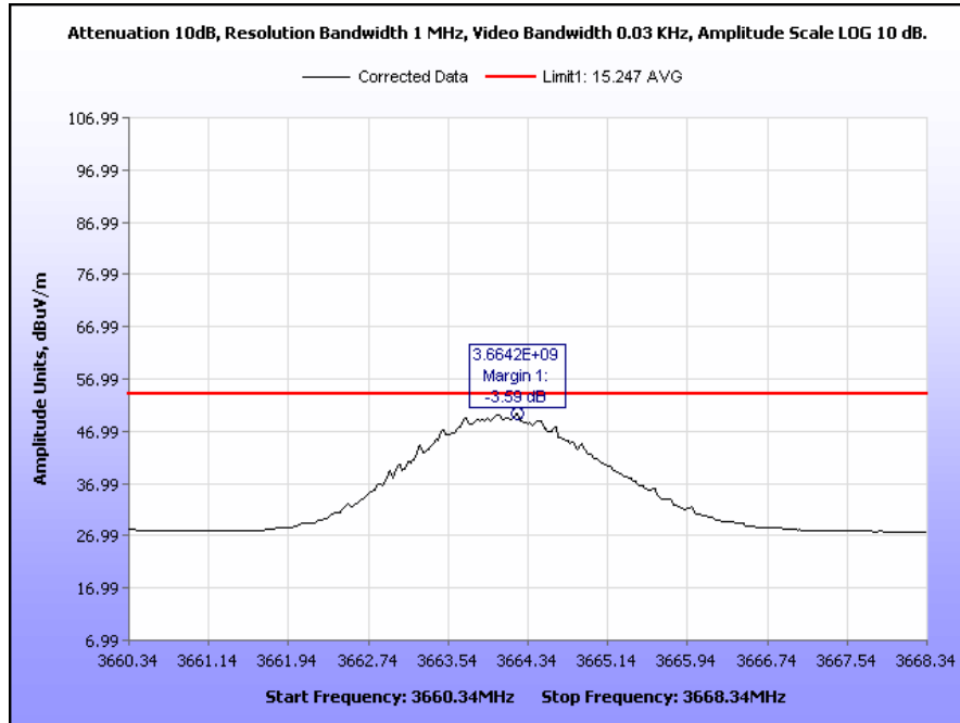
Plot 21. Transmitter Spurious Emissions, Mid Channel, 3 GHz – 6 GHz, Average
