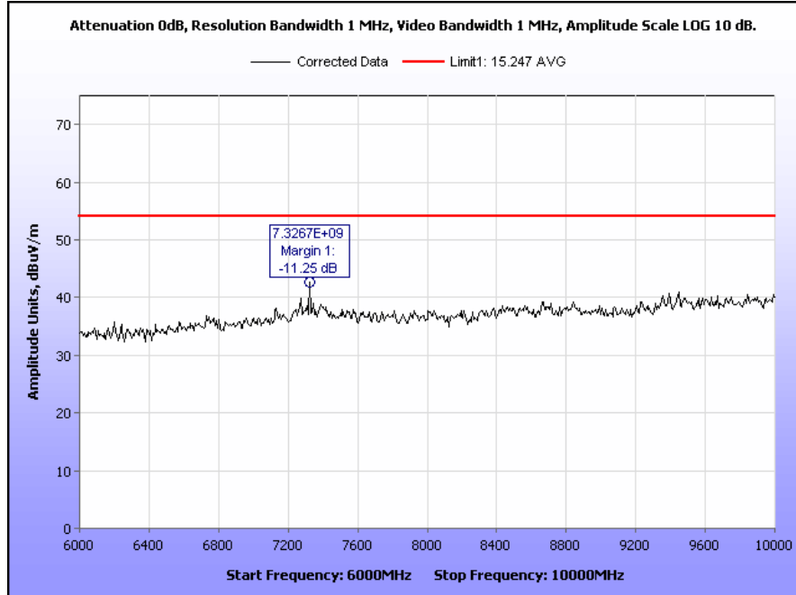
Plot 22. Transmitter Spurious Emissions, Mid Channel, 6 GHz – 10 GHz
