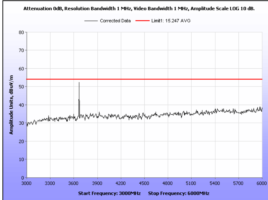
Plot 20. Transmitter Spurious Emissions, Mid Channel, 3 GHz – 6 GHz
