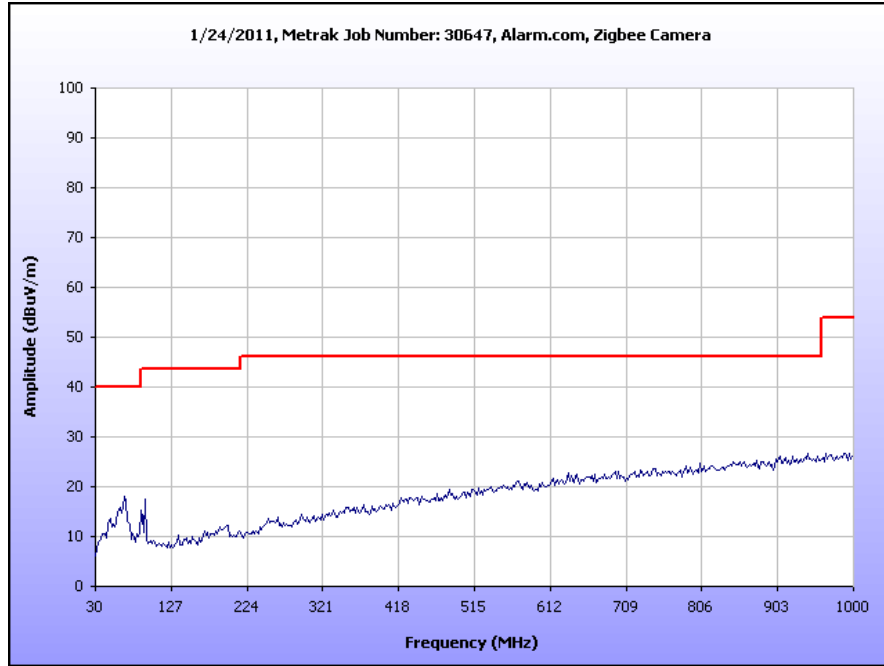
Plot 28. Receiver Spurious Emission, 30 MHz – 1 GHz
