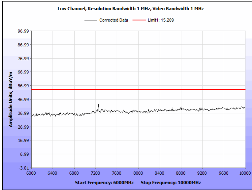
Plot 17. Transmitter Spurious Emissions, Low Channel, 6 GHz – 10 GHz
