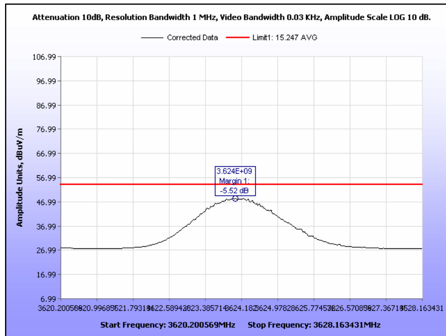
Plot 16. Transmitter Spurious Emissions, Low Channel, 3 GHz – 6 GHz, Average
