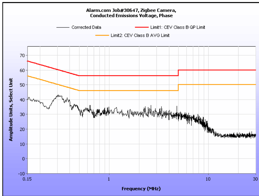
Plot 5. 15.207 Conducted Emissions, Phase Line
