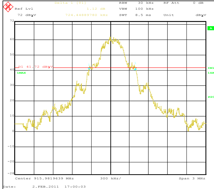
Plot 11. 99% Occupied Bandwidth, Mid Channel
