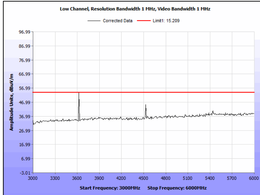
Plot 15. Transmitter Spurious Emissions, Low Channel, 3 GHz – 6 GHz
