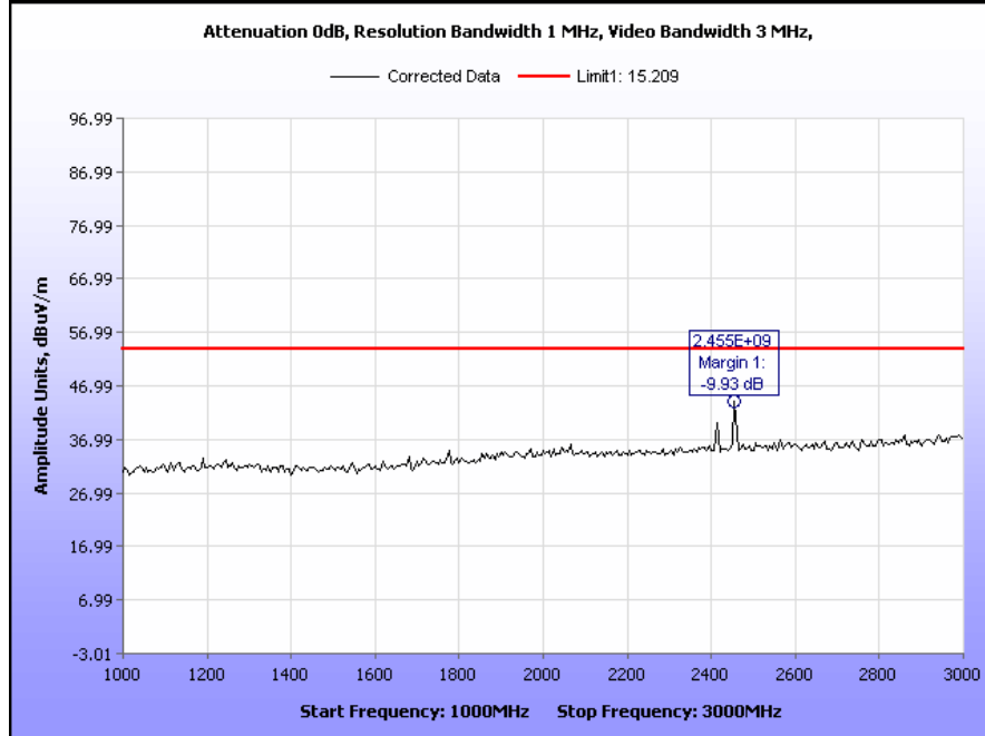
Plot 29. Receiver Spurious Emission, 1 GHz – 3 GHz
