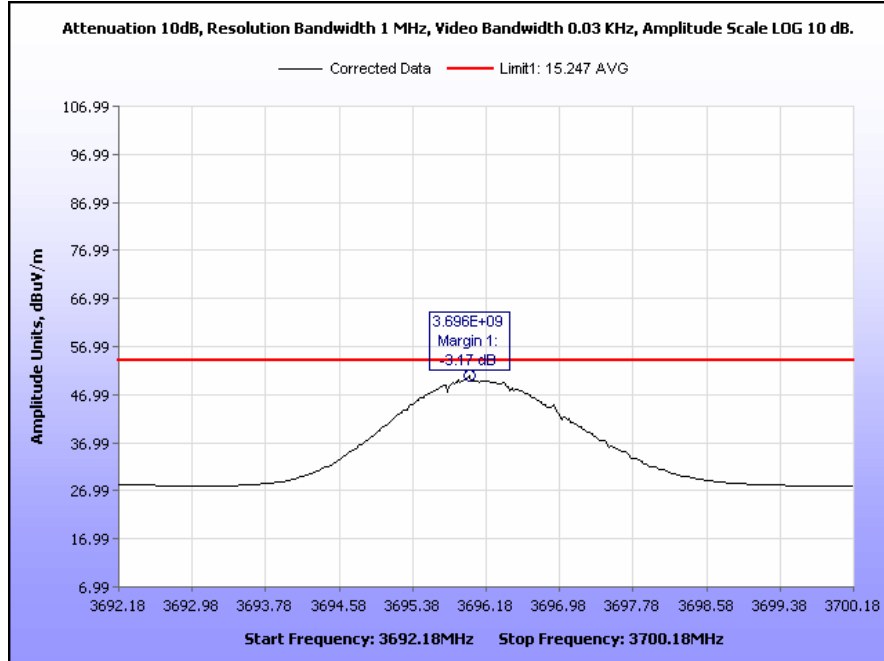
Plot 26. Transmitter Spurious Emissions, High Channel, 3 GHz – 6 GHz, Average
