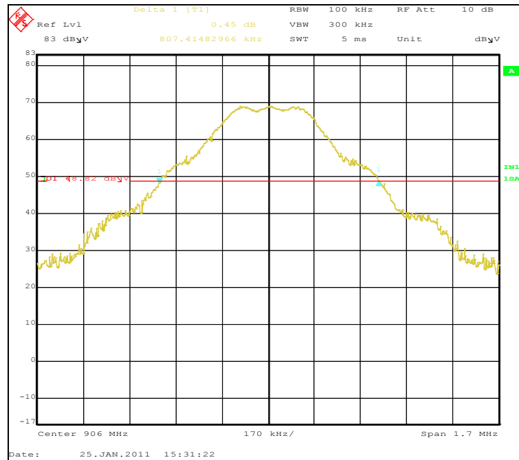
Plot 7. Occupied Bandwidth, Low Channel
