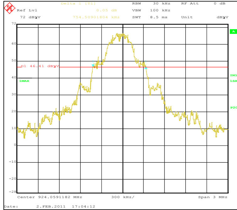
Plot 12. 99% Occupied Bandwidth, High Channel
