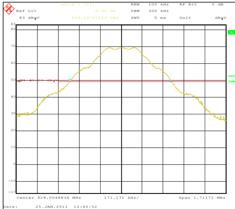
Plot 9. Occupied Bandwidth, High Channel
