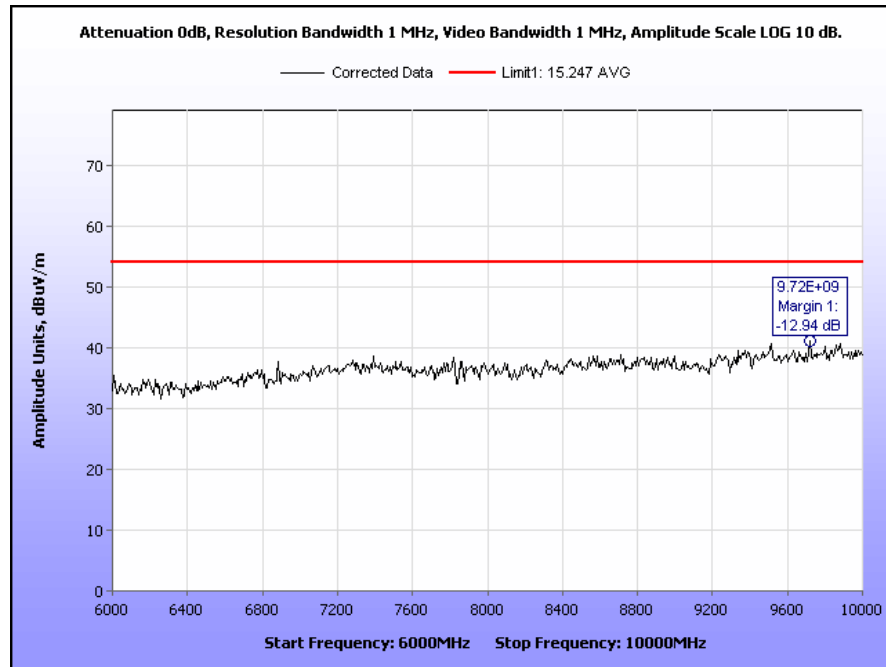
Plot 27. Transmitter Spurious Emissions, High Channel, 6 GHz – 10 GHz
