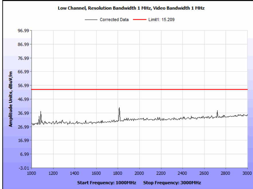
Plot 14. Transmitter Spurious Emissions, Low Channel, 1 GHz – 3 GHz
