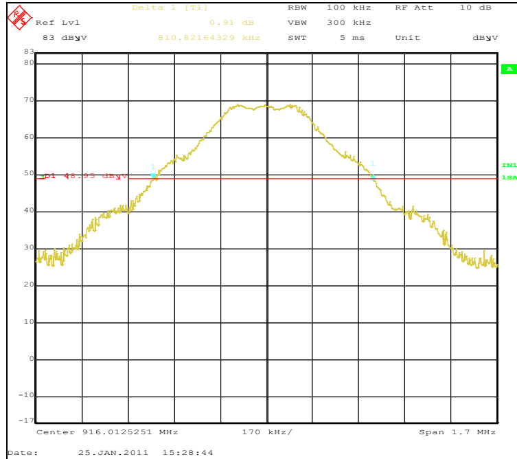
Plot 8. Occupied Bandwidth, Mid Channel
