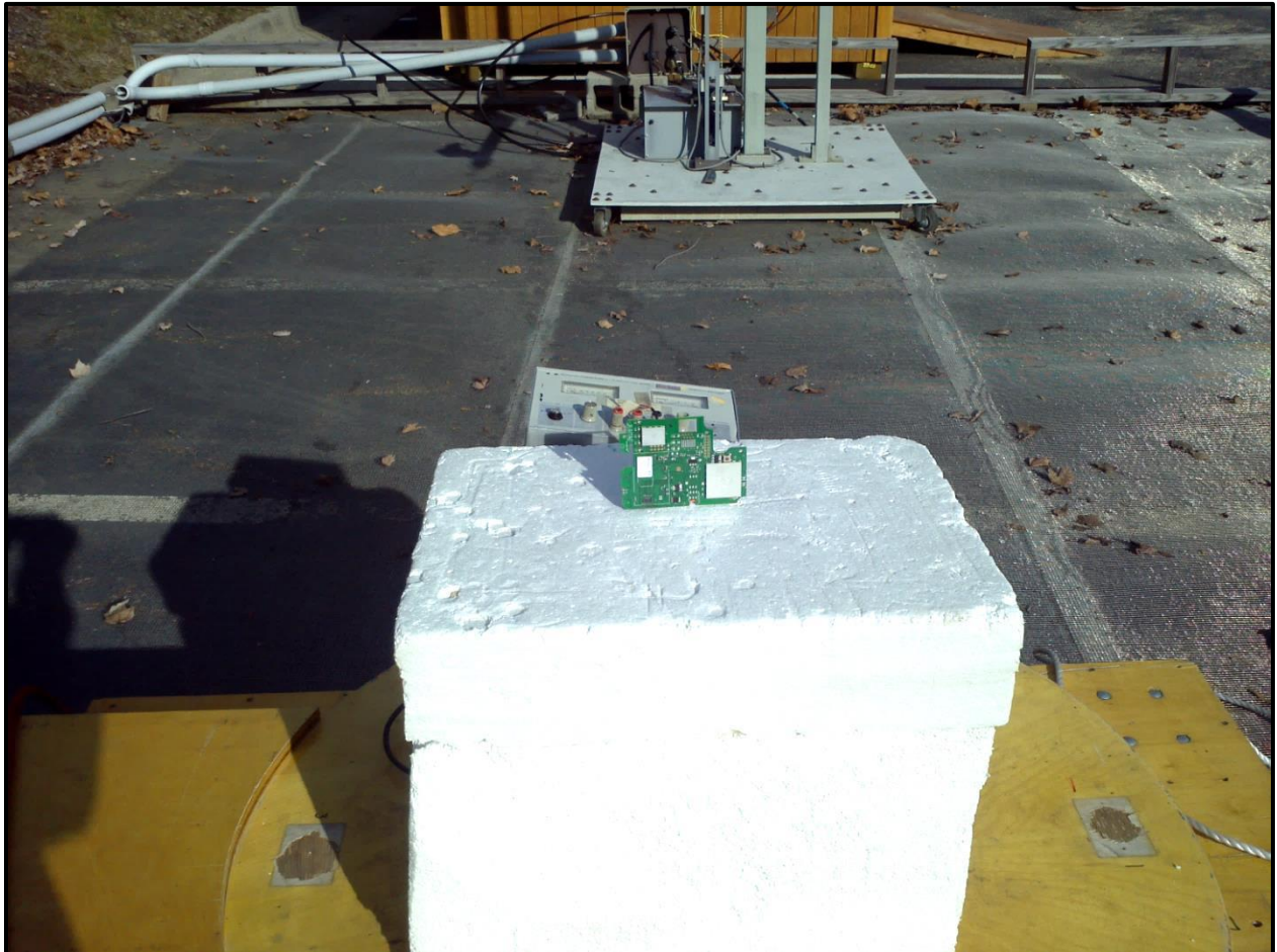
Photograph 2: Radiated Emissions Testing – Front View
