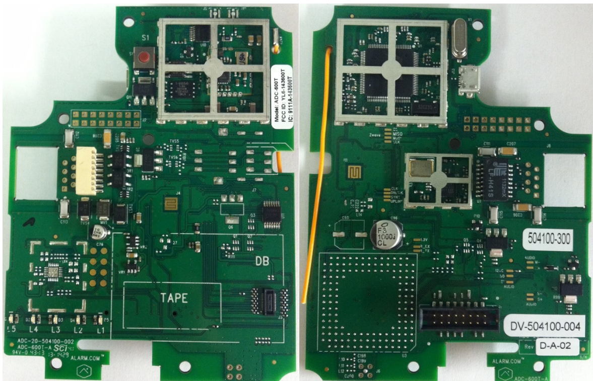
Model ADC-600T Top and Bottom view without shields and FCC/IC label location.
