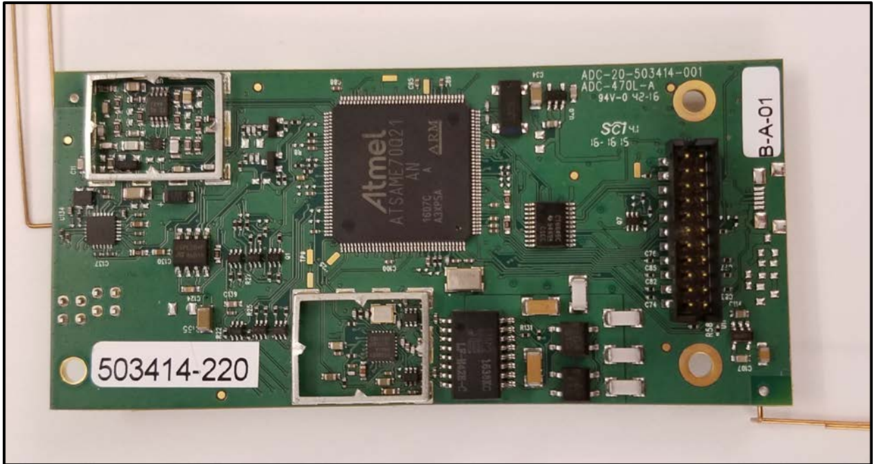
Photograph 13: Module Bottom View – No Shields
