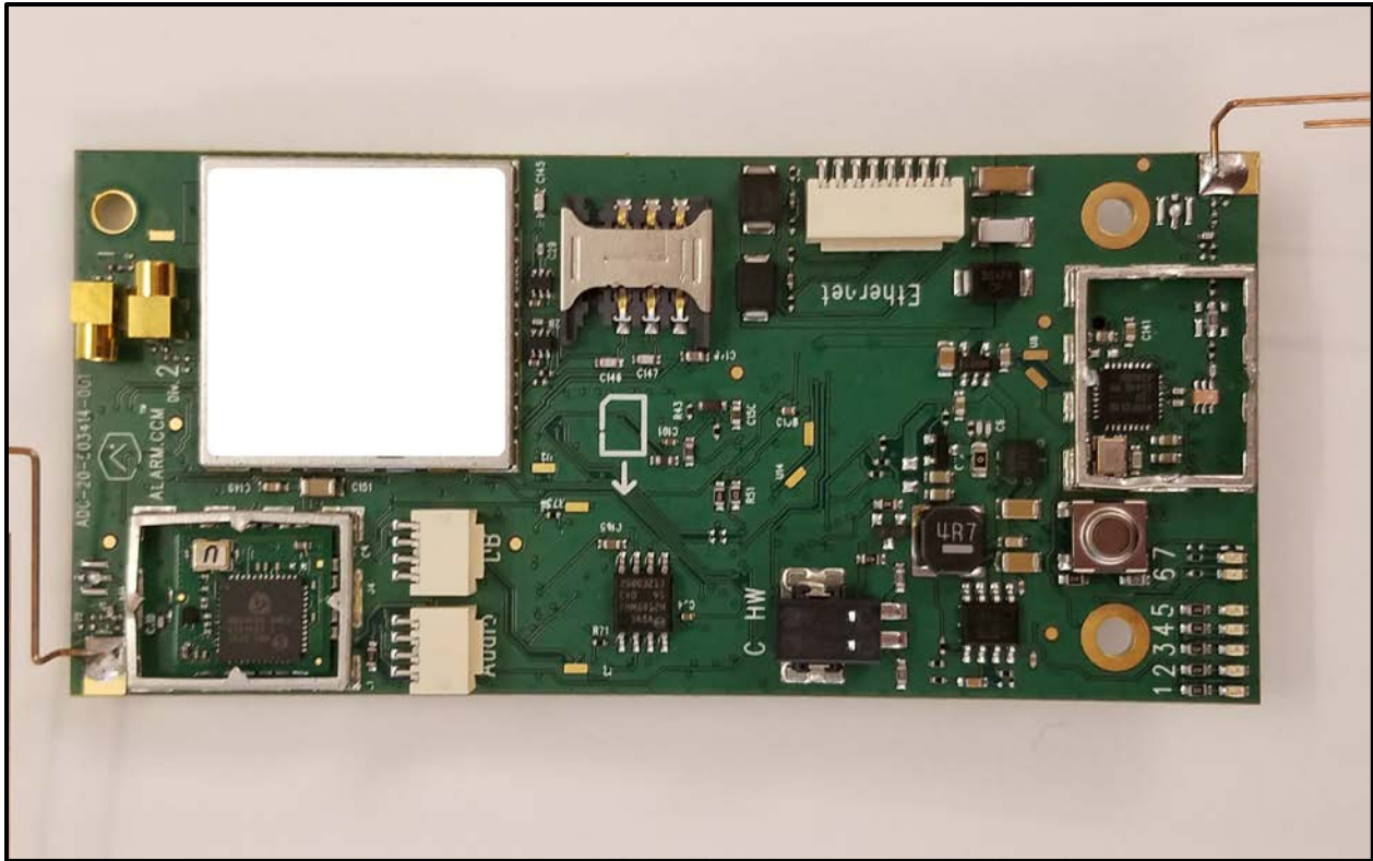
Photograph 8: Module Top View – No Shields
