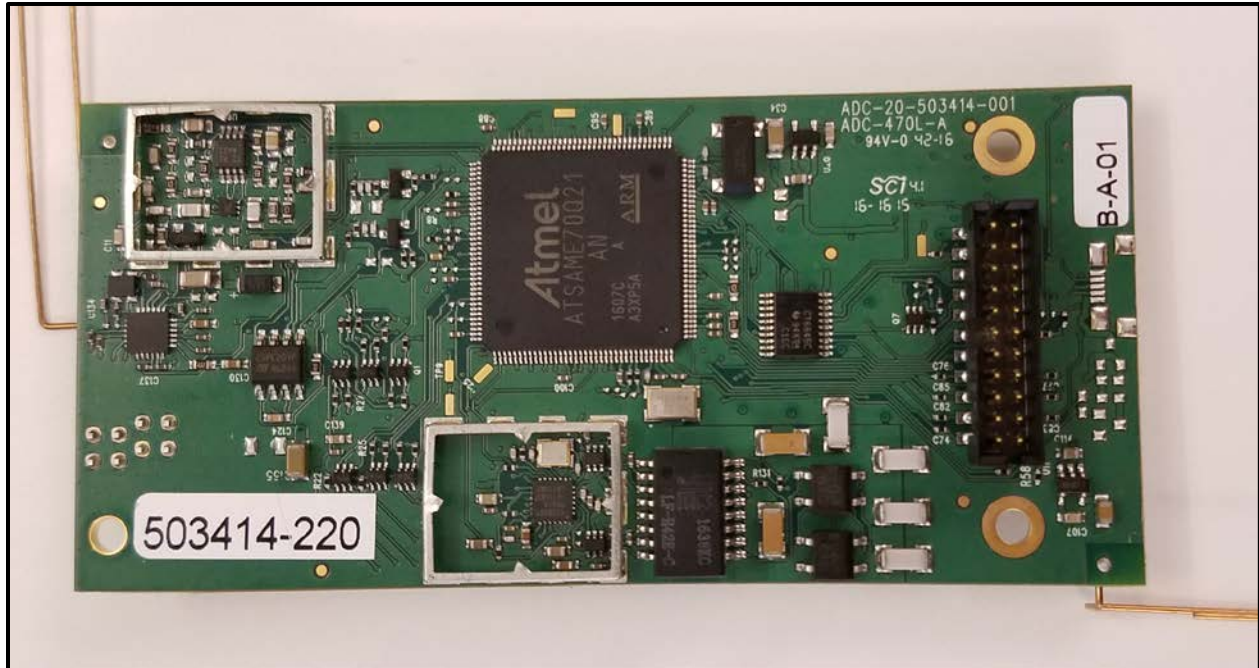
Photograph 9: Module Bottom View – No Shields
