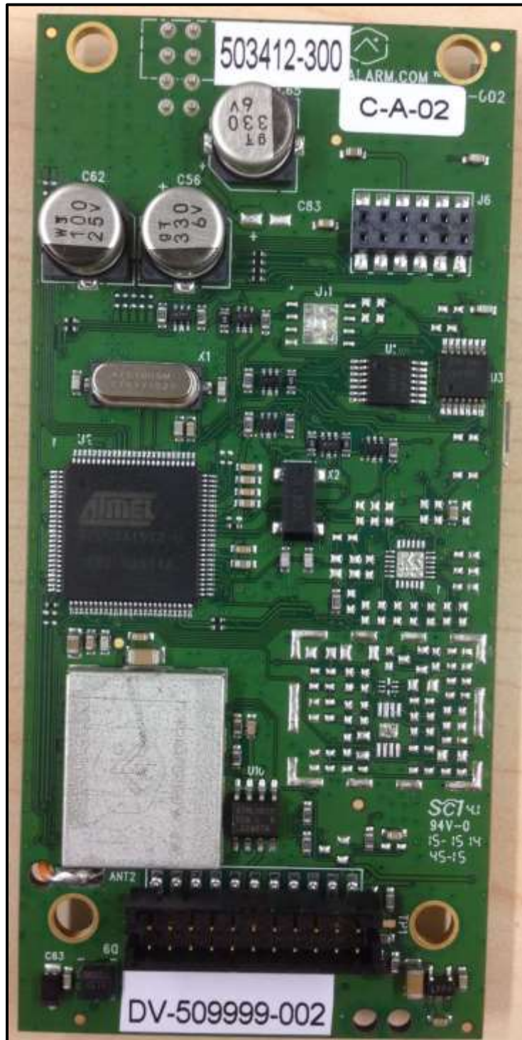
Photograph 19: PCB Bottom with Shield
