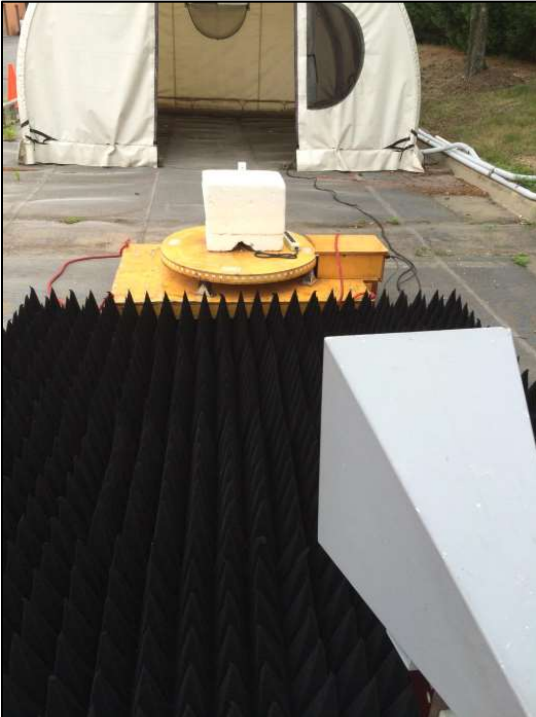
Photograph 2: Radiated Emissions Testing – Front View (with cones)
