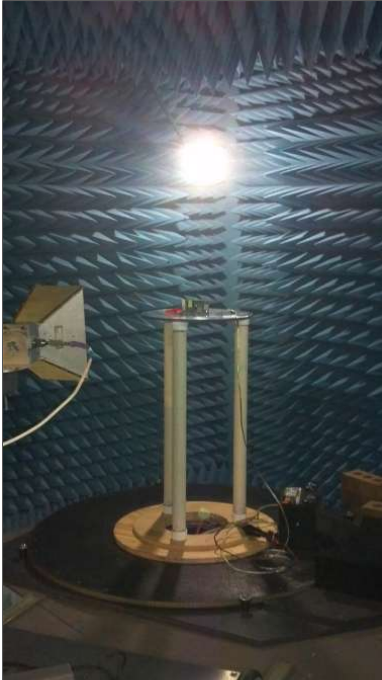
Photograph 2. Radiated Spurious Emissions, Test Setup
