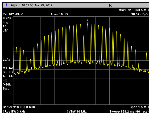
Plot 27. Peak Power Spectral Density, Mid Channel, Peak Determination
