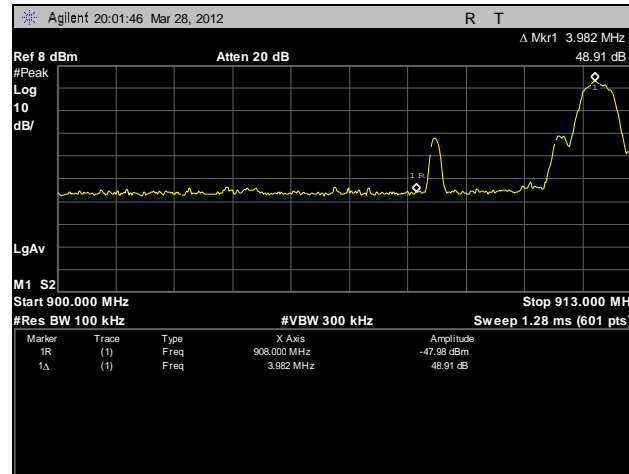
Plot 20. 20 dBc Band Edge, Low Channel
