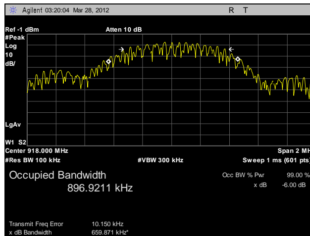
Plot 3. 6 dB Occupied Bandwidth, Mid Channel
