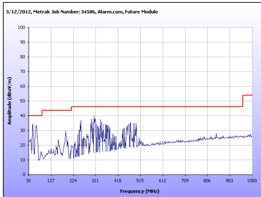
Plot 1. Radiated Emissions, 30 MHz - 1 GHz, FCC Limits, Radio Off
