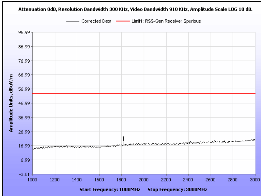
Plot 32. Receiver Spurious Emission, 1 GHz – 3 GHz
