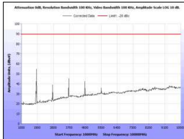
Plot 23. Radiated Spurious Emissions, Mid Channel
