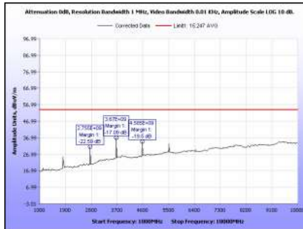
Plot 16. Radiated Spurious Emissions, Mid Channel, 1 GHz – 10 GHz, Average
