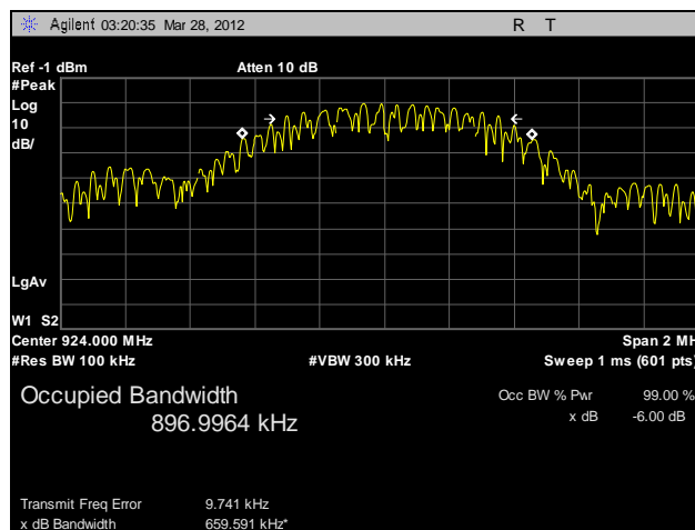
Plot 4. 6 dB Occupied Bandwidth, High Channel
