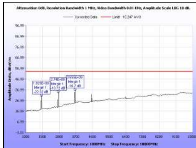
Plot 13. Radiated Spurious Emissions, Low Channel, 1 GHz – 10 GHz, Average
