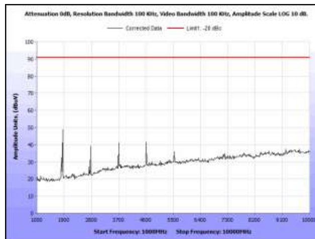
Plot 24. Radiated Spurious Emissions, High Channel
