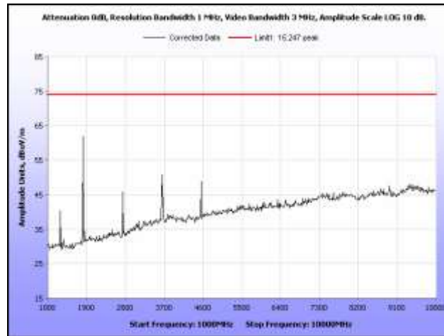
Plot 12. Radiated Spurious Emissions, Low Channel, 1 GHz – 10 GHz, Peak
