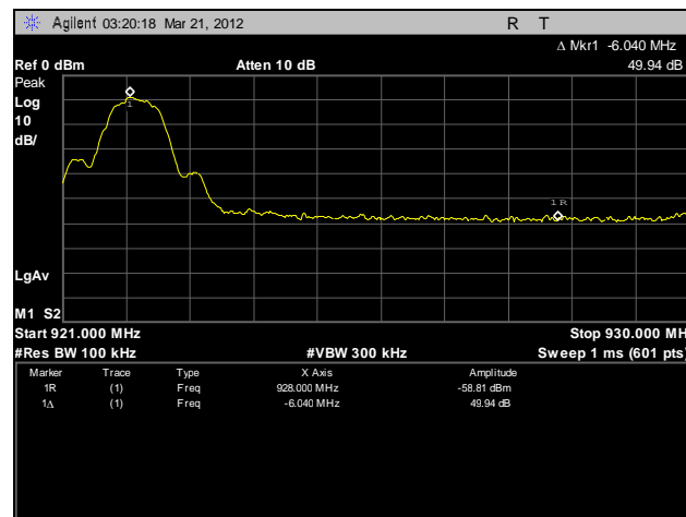
Plot 21. 20 dBc Band Edge, High Channel
