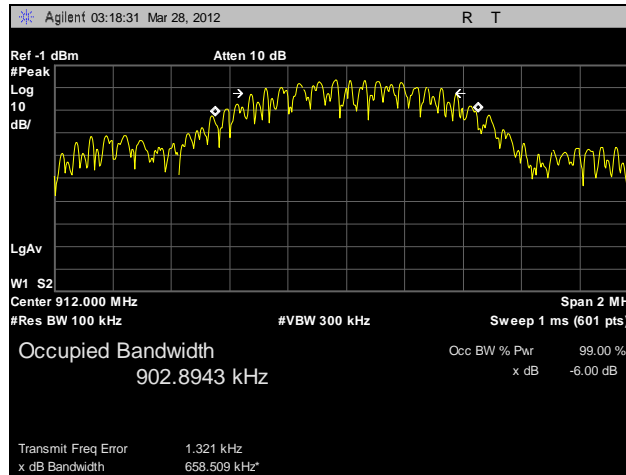
Plot 2. 6 dB Occupied Bandwidth, Low Channel
