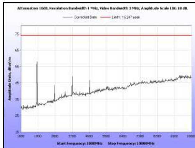
Plot 18. Radiated Spurious Emissions, High Channel, 1 GHz – 10 GHz, Peak
