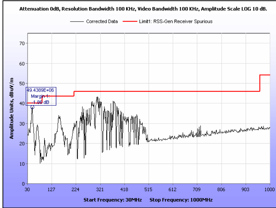
Plot 31. Receiver Spurious Emission, 30 MHz – 1 GHz
