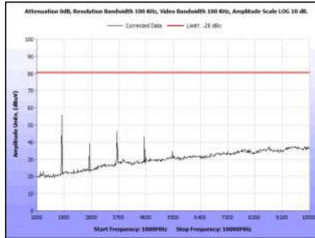
Plot 22. Radiated Spurious Emissions, Low Channel
