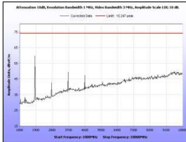
Plot 15. Radiated Spurious Emissions, Mid Channel, 1 GHz – 10 GHz, Peak
