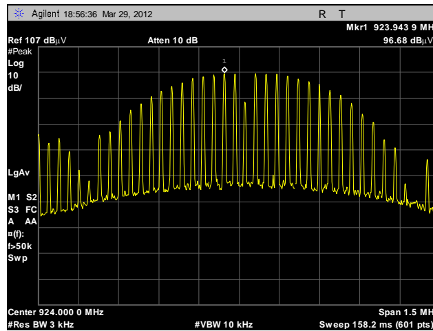
Plot 29. Peak Power Spectral Density, High Channel, Peak Determination
