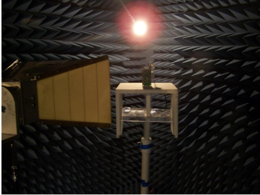
Photograph 3. Radiated Harmonics, Test Setup
