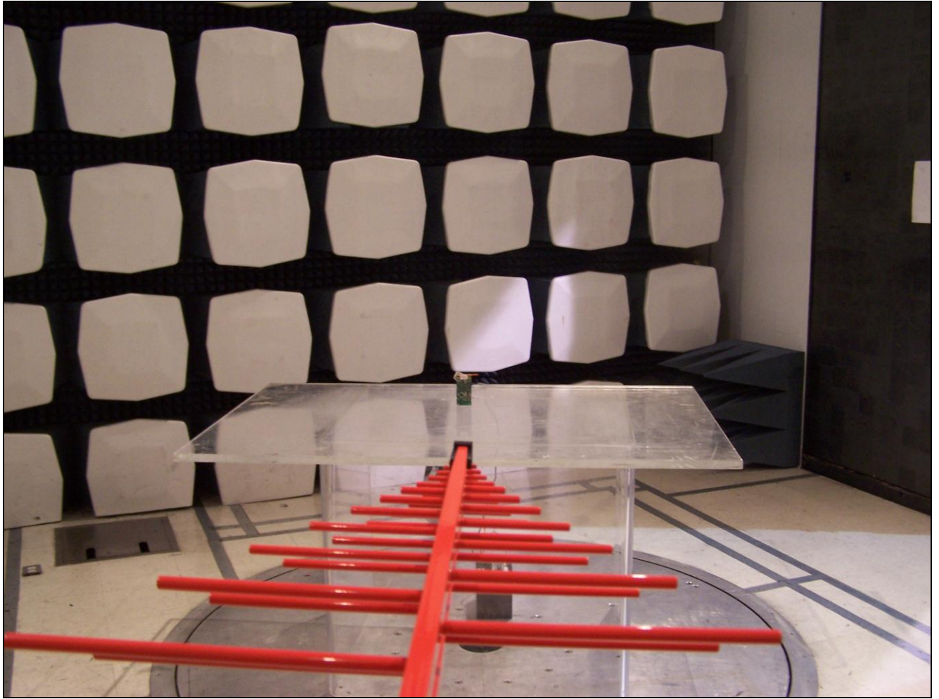
Photograph 2. Radiated Field Strength of Fundamental, Test Setup
