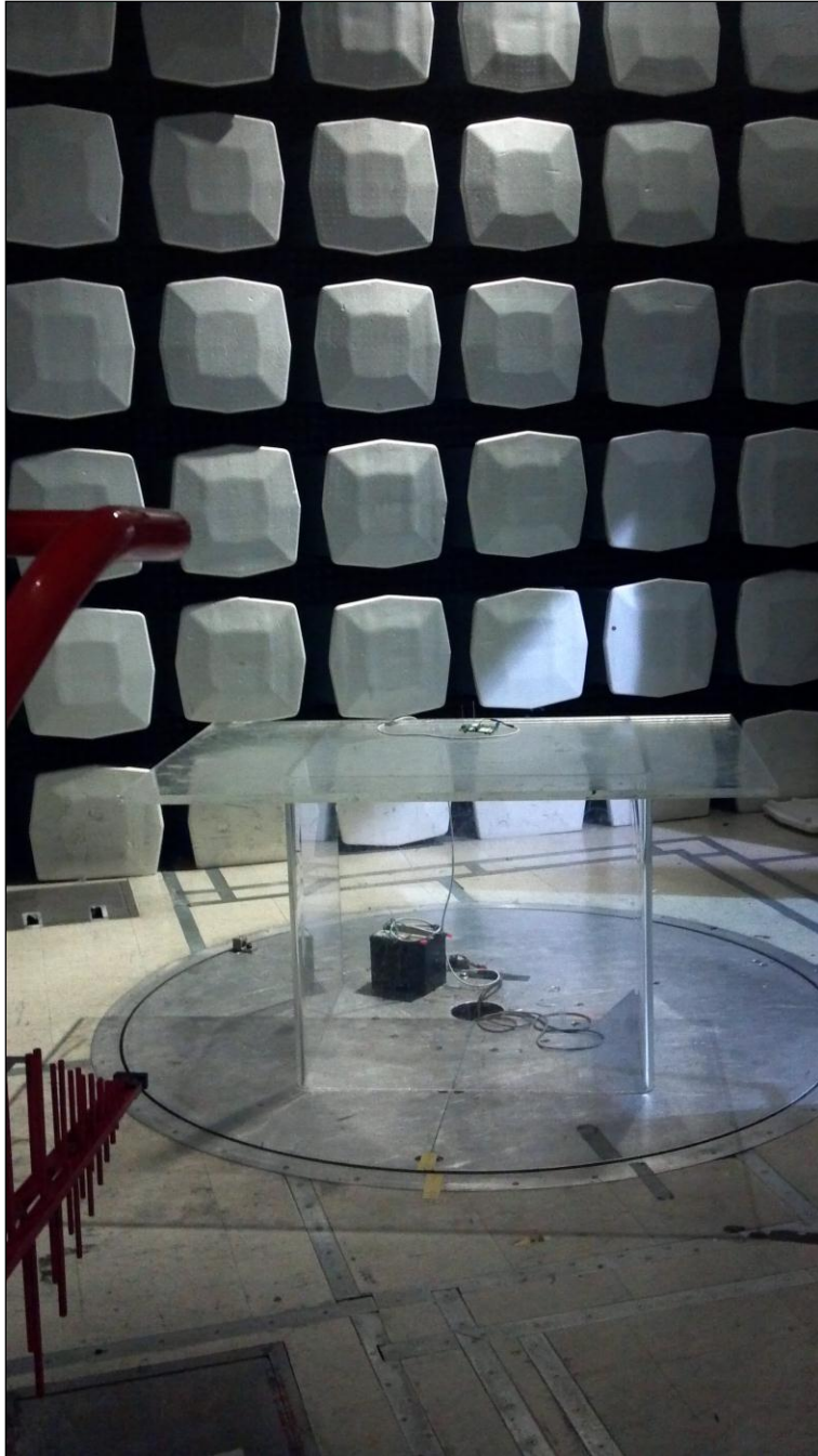
Photograph 2. Radiated Spurious Emissions, Test Setup, 30 MHz – 1 GHz
