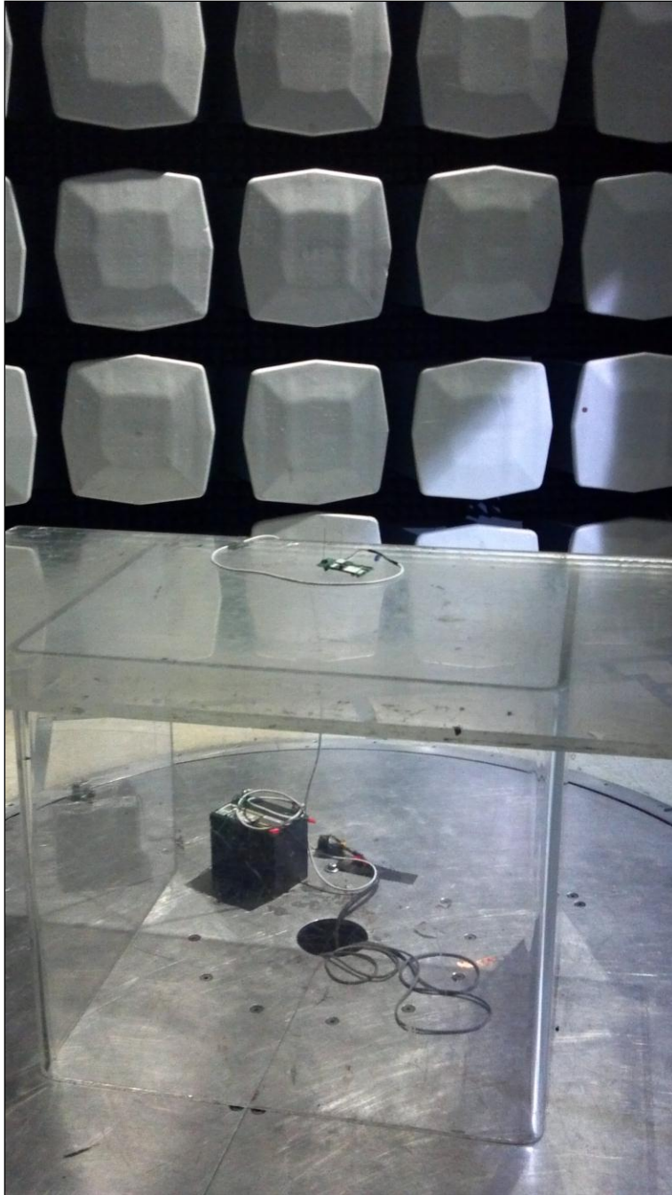
Photograph 1. Radiated Emissions, Test Setup
