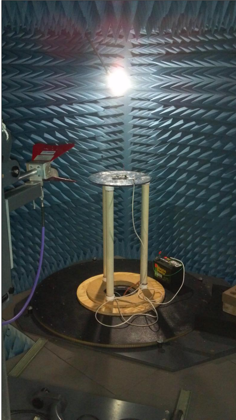
Photograph 3. Radiated Spurious Emissions, Test Setup, Above 1 GHz
