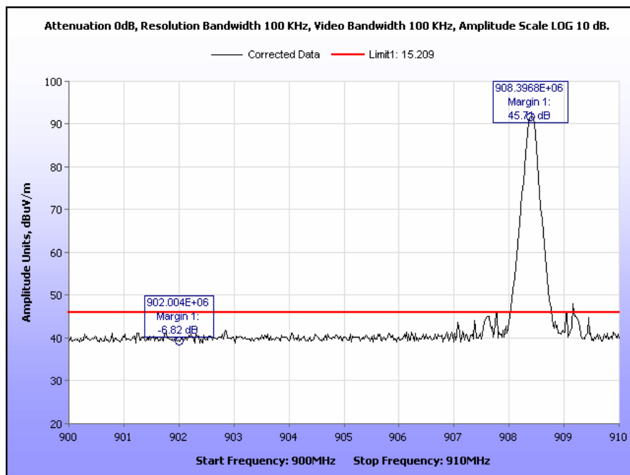
Plot 5. Radiated Field Strength, Band Edge, Low End
