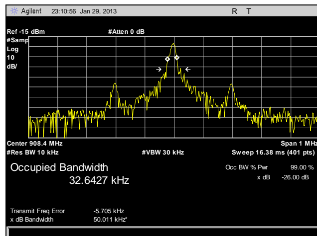
Plot 4. 99% Occupied Bandwidth
