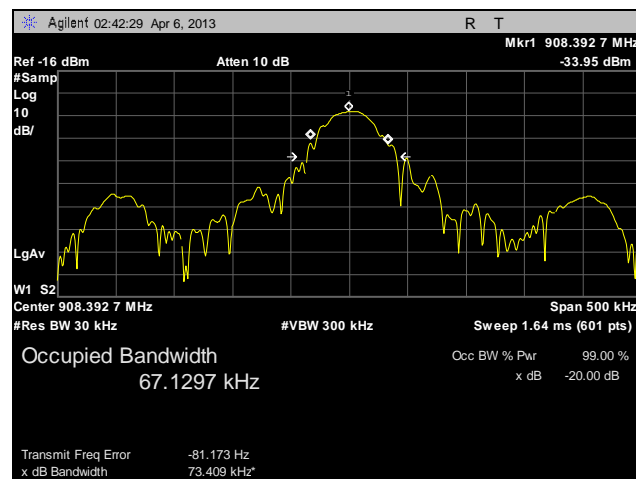
Plot 3. Occupied Bandwidth
