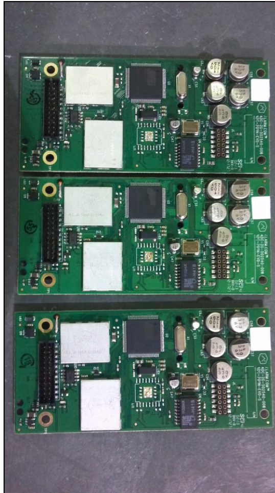
Photograph 1. Novatel CDMA Module; Model: ADC-200N-EVD
