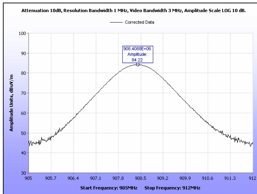
Plot 2. Radiated Field Strength, 908 MHz Fundamental
