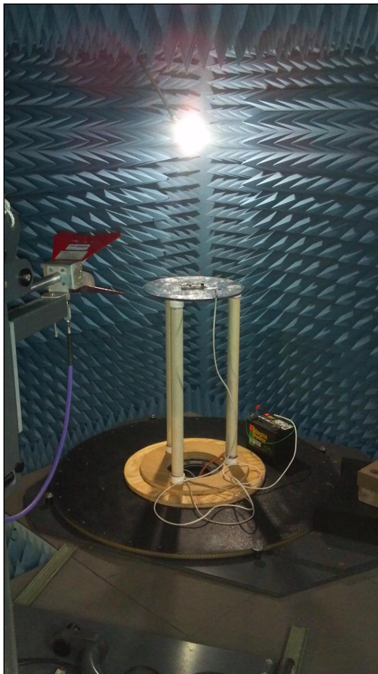
Photograph 4. Radiated Spurious Emissions, Test Setup, Above 1 GHz
