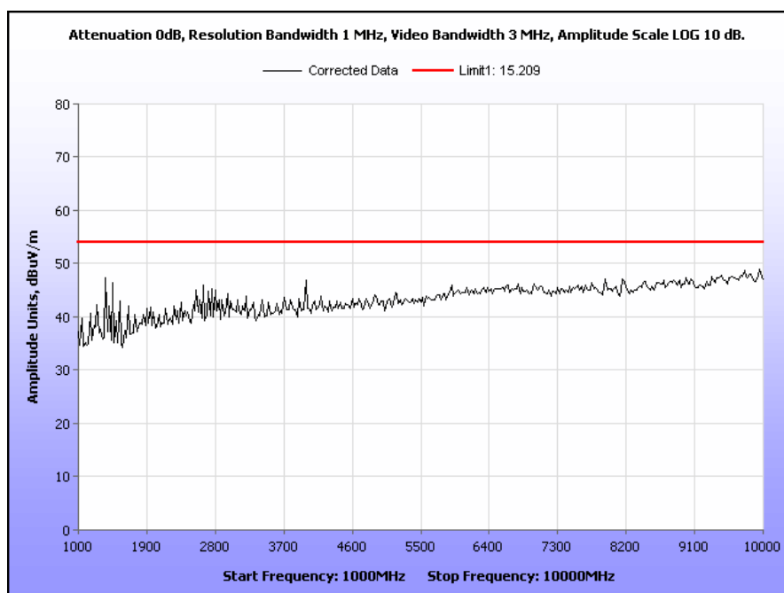
Plot 8. Radiated Spurious Emissions, 1 GHz – 10 GHz, Peak Under Average Limit
