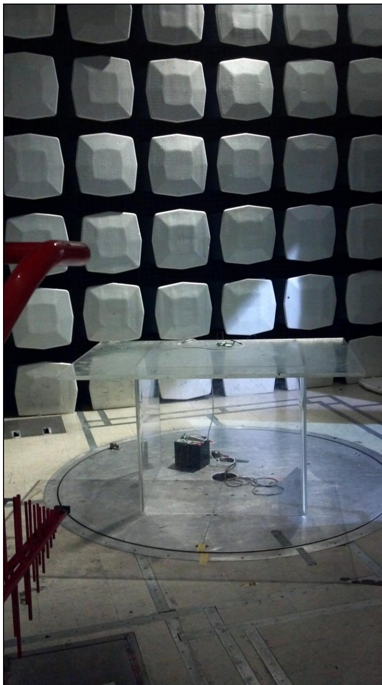
Photograph 3. Radiated Spurious Emissions, Test Setup, 30 MHz – 1 GHz
