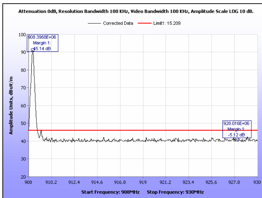
Plot 6. Radiated Field Strength, Band Edge, High End
