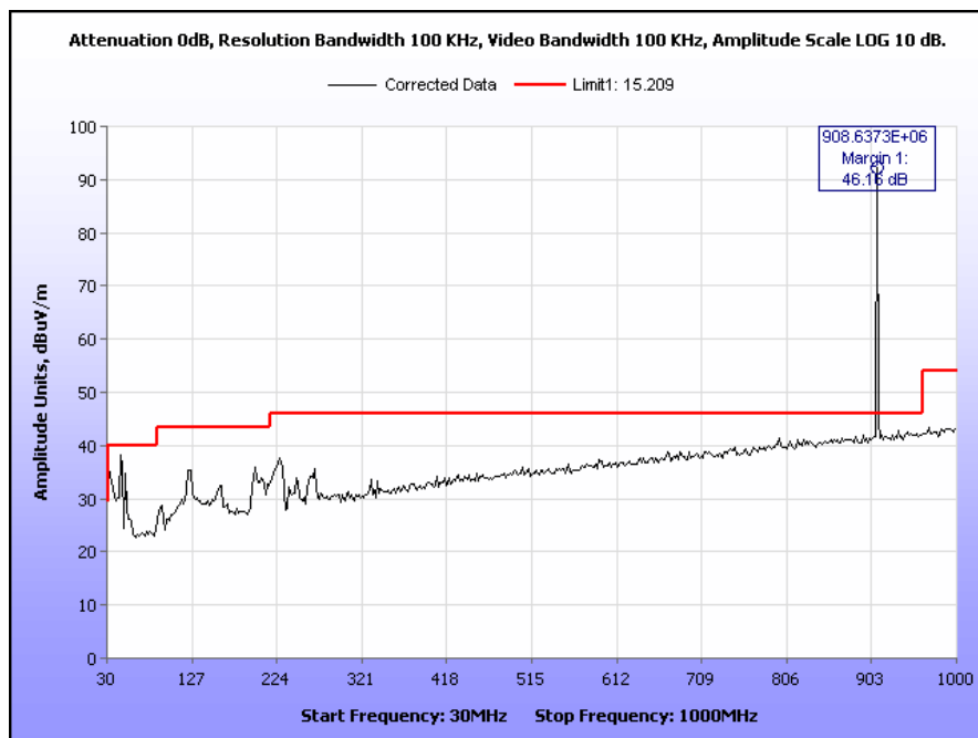
Plot 7. Radiated Spurious Emissions, 30 MHz – 1 GHz, Transmitter On
