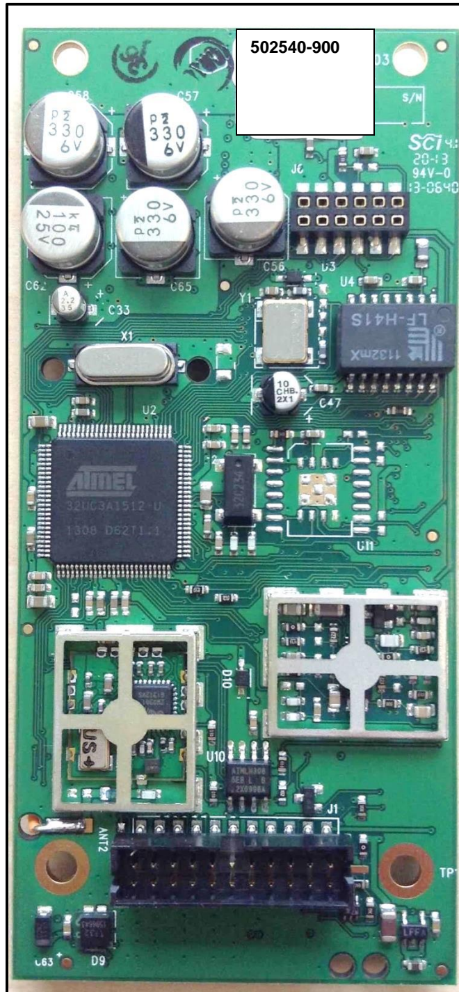
Photograph 8: Variant 502540-900 Bottom View without Shields
