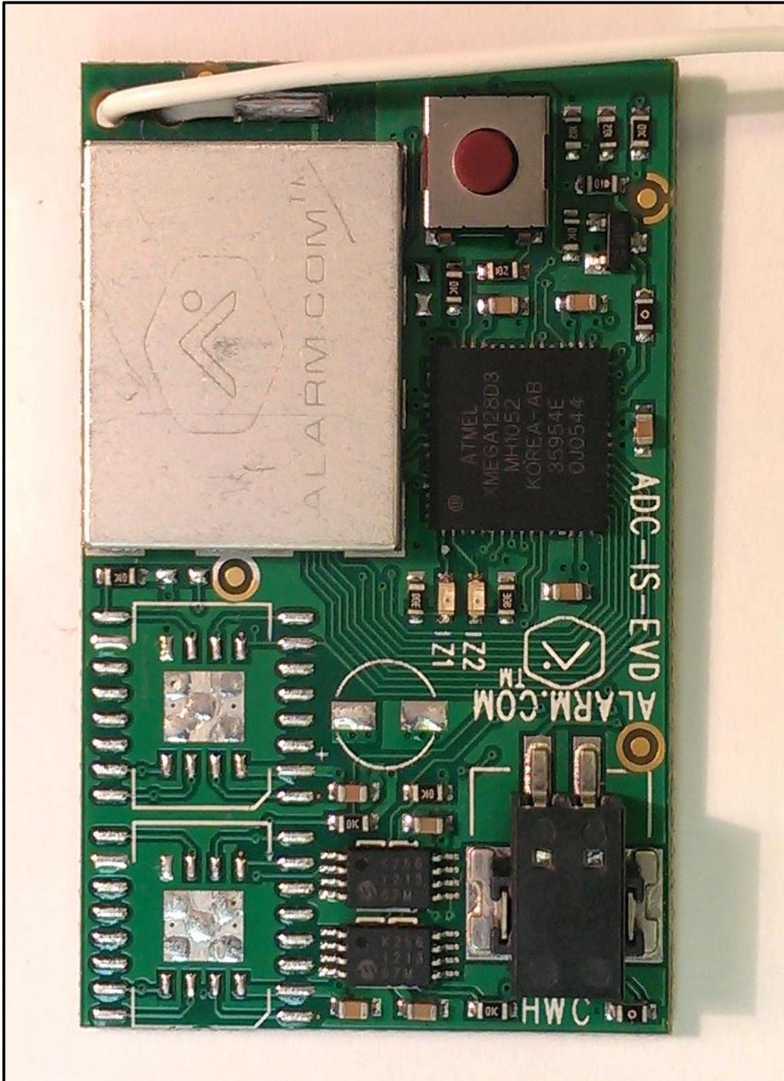
Photograph 11: Module FCC ID: YL6-143IS205V4 – Front View
