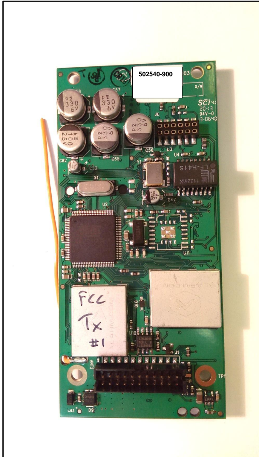
Photograph 7: Variant 502540-900 Bottom View with Shields
