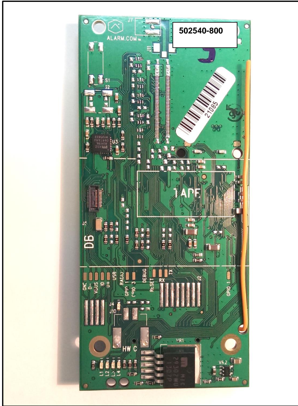
Photograph 9: Variant 502540-800 Top View
