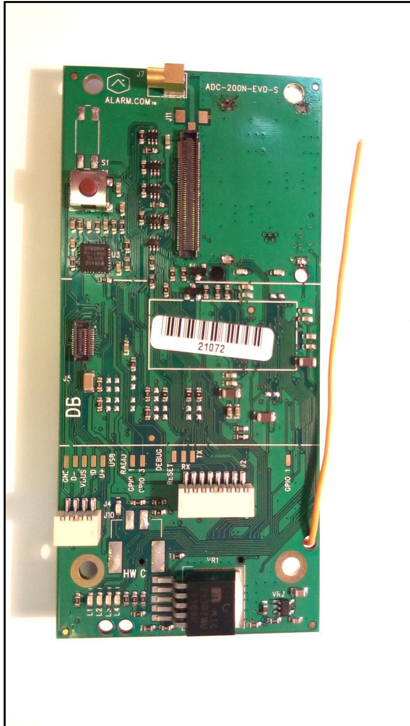
Photograph 6: Variant 502540-900 Top View without FCC ID: YL6-143IS205V4
