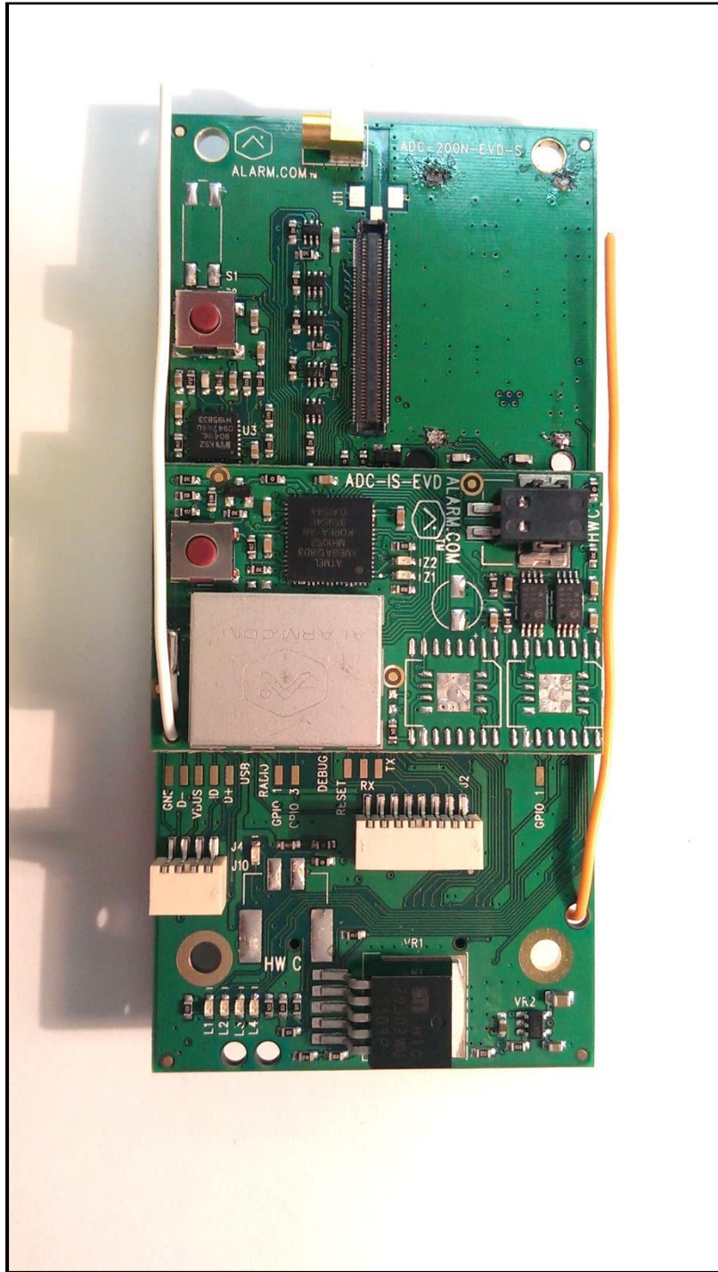
Photograph 5: Variant 502540-900 with FCC ID: YL6-143IS205V4 Module
