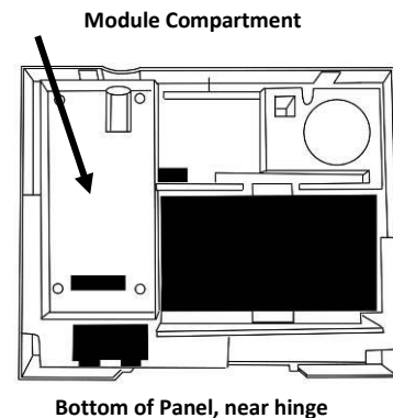
Figure 2: Module compartment
