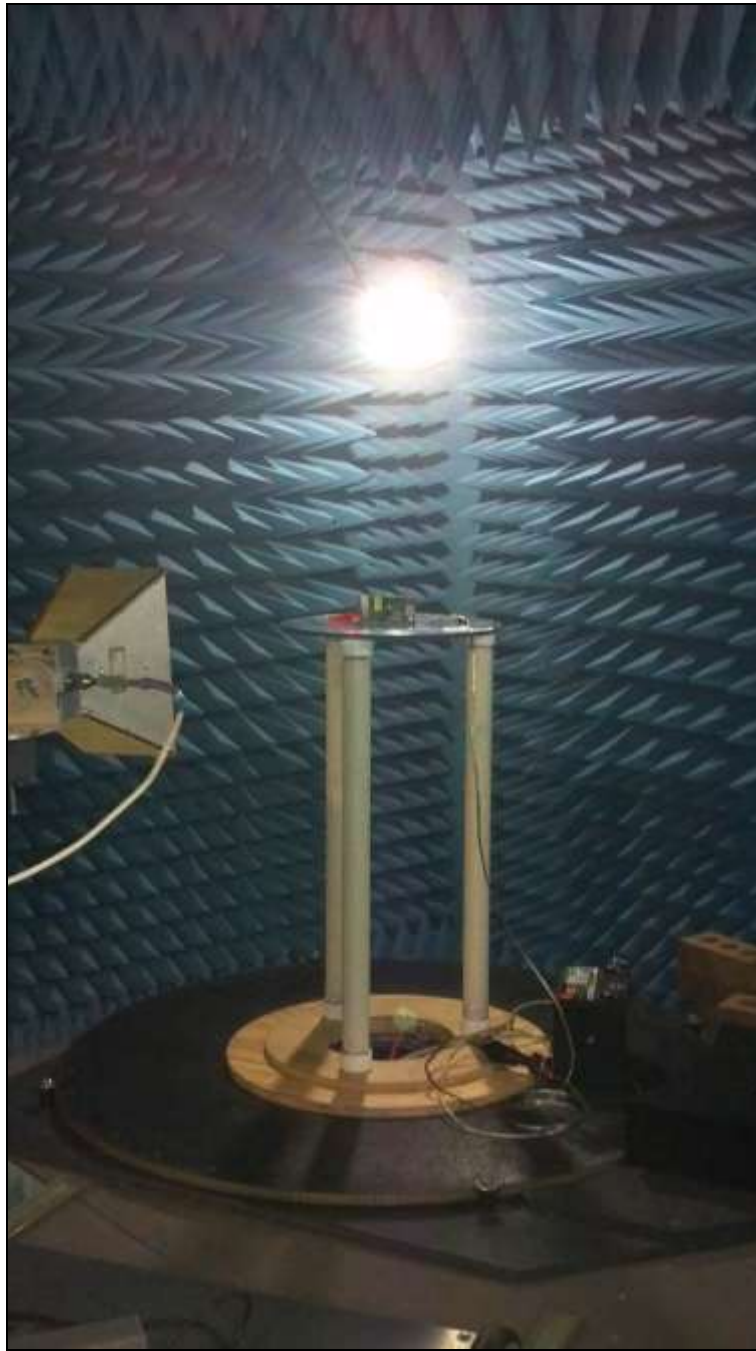
Photograph 2. Radiated Spurious Emissions, Test Setup
