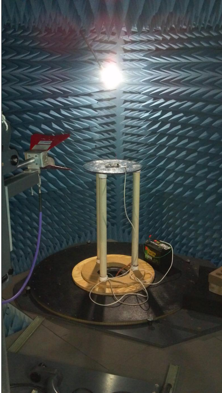
Photograph 1. Collocation Test Setup, 1
