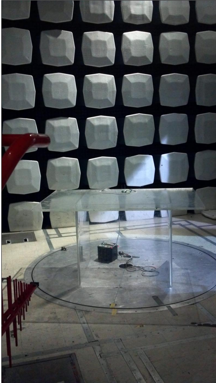
Photograph 2. Collocation Test Setup, 2
