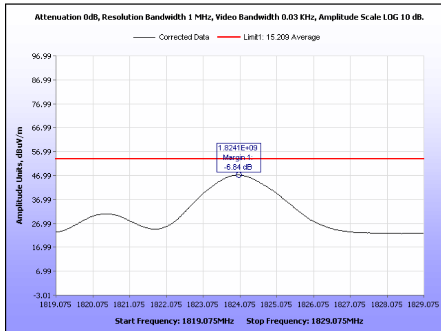
Plot 4. Transmitter Spurious Emissions, Low Channel, 1824 MHz, Average
