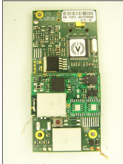
Photograph 1. ADC-200C-EVD Wireless Module Collocated with ADC-IS20-EVD Wireless Module
