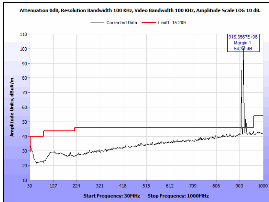
Plot 6. Radiated Spurious Emissions, Mid Channel, 30 MHz – 1 GHz
