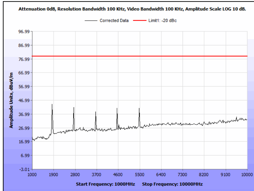
Plot 5. Transmitter Spurious Emissions, Low Channel, 100 kHz, RBW
