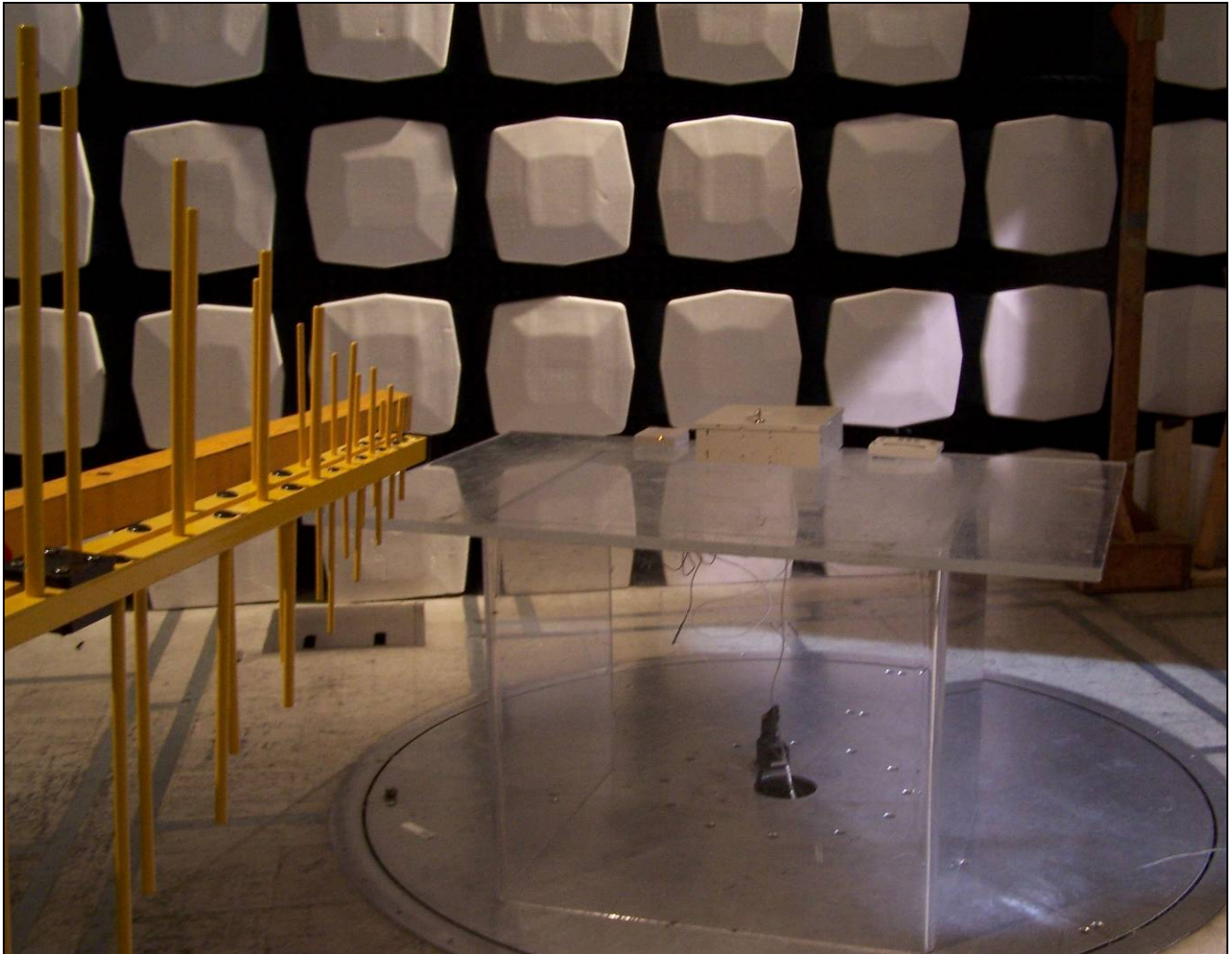
Photograph 4. Radiated Emissions, Test Setup
