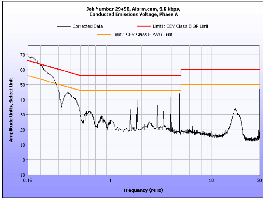
Plot 4. Conducted Emissions, Phase Line, 9.6 kbps
