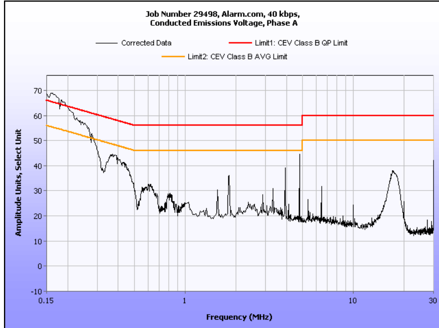
Plot 5. Conducted Emissions, Phase Line, 40 kbps
