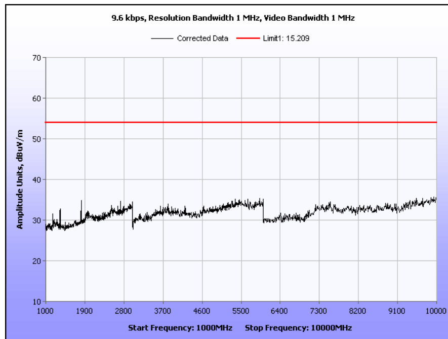
Plot 8. Radiated Harmonics, 9.6kpbs, 1 GHz – 10 GHz
