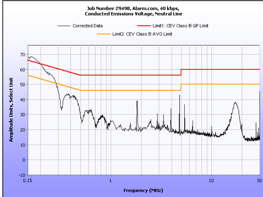
Plot 7. Conducted Emissions, Neutral Line, 40 kbps
