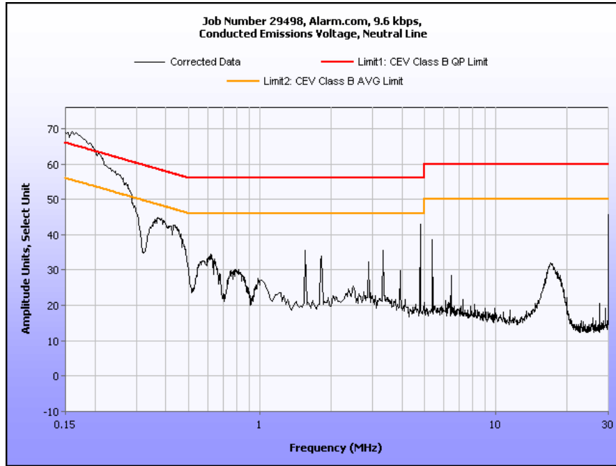
Plot 6. Conducted Emissions, Neutral Line, 9.6 kbps
