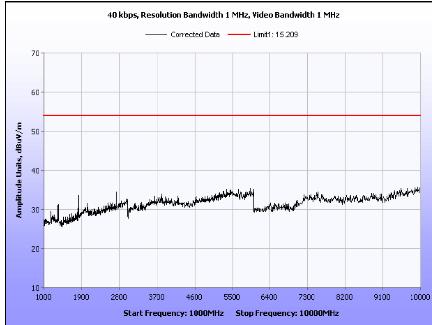
Plot 9. Radiated Harmonics, 40 kbps, 1 GHz – 10 GHz
