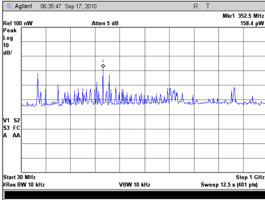
Plot 6. Receiver Spurious Emission, 30 MHz – 1 GHz
