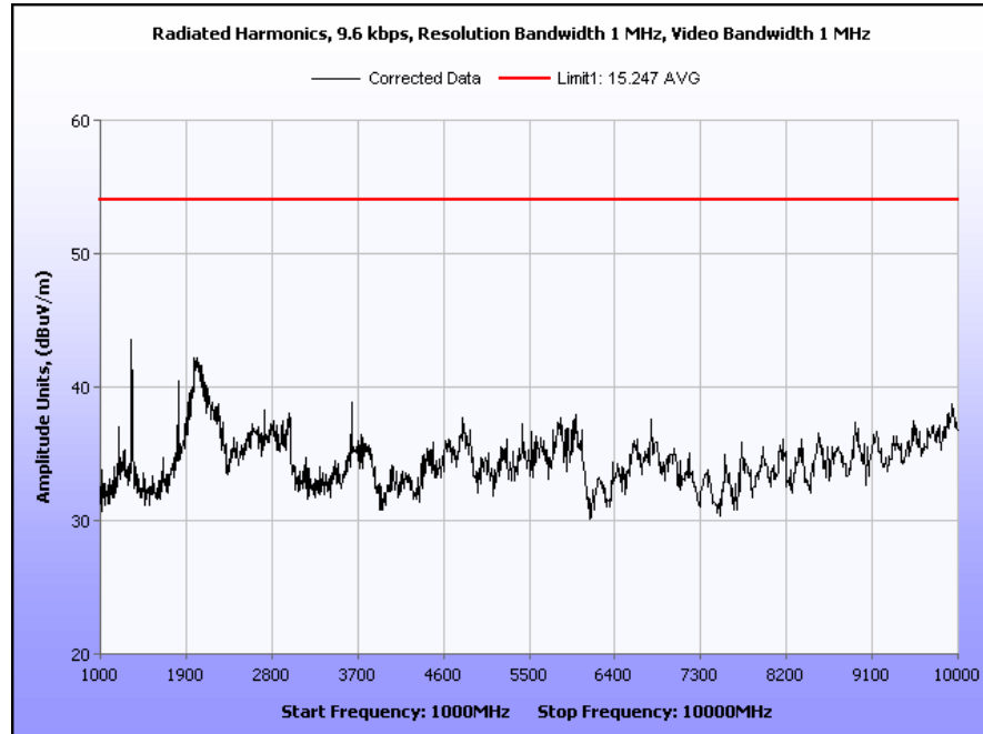
Plot 4. Radiated Harmonics, 9.6kBPS, 1 GHz – 10 GHz
