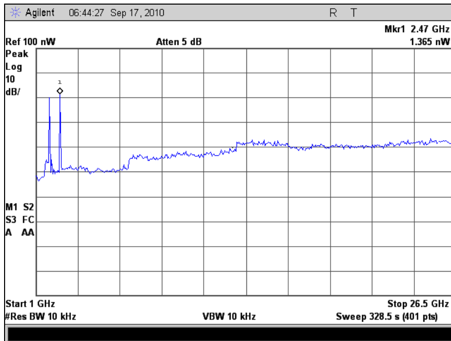
Plot 7. Receiver Spurious Emission, 1 GHz – 26.5 GHz
