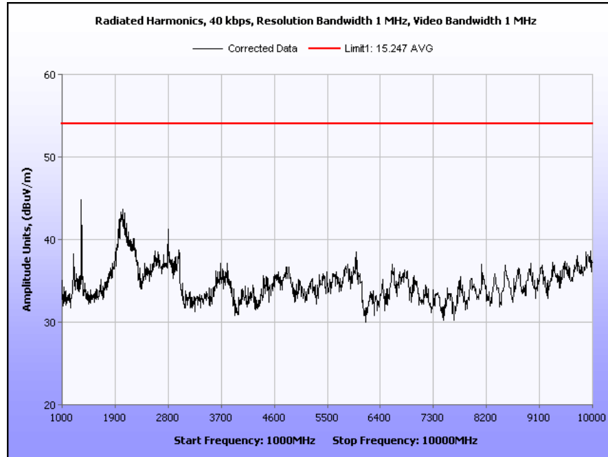
Plot 5. Radiated Harmonics, 40 kbps, 1 GHz – 10 GHz
