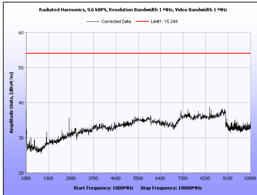
Plot 16. Radiated Harmonics, Hosting Device, 9.6 kbps, 902 – 928 MHz Frequency
