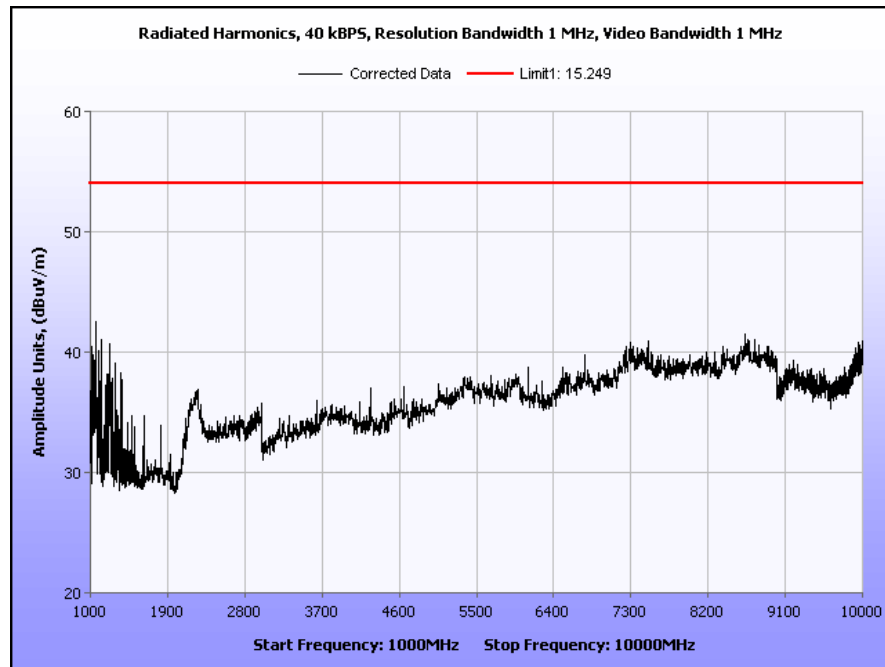
Plot 13. Radiated Harmonics, 40 kbps, 1 GHz – 10 GHz
