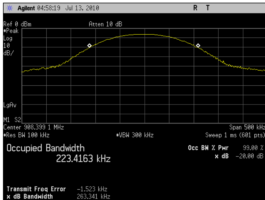
Plot 10. Occupied Bandwidth, FCC Limits
