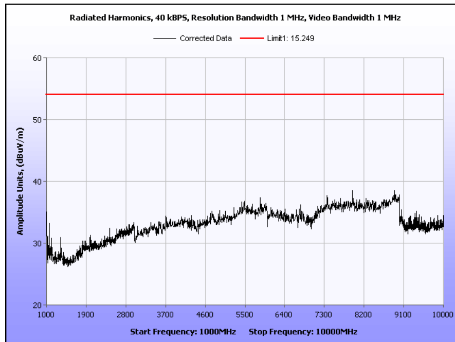
Plot 17. Radiated Harmonics, Hosting Device, 40 kbps, 902 – 928 MHz Frequency
