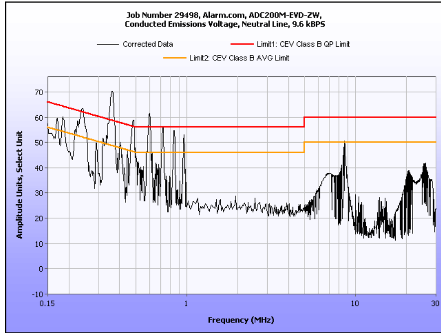
Plot 7. Conducted Emissions, Neutral Line, 9.6 kBPS
