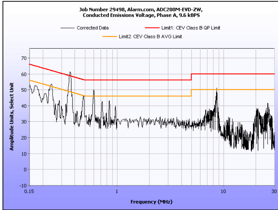
Plot 5. Conducted Emissions, Phase Line, 9.6 kbps
