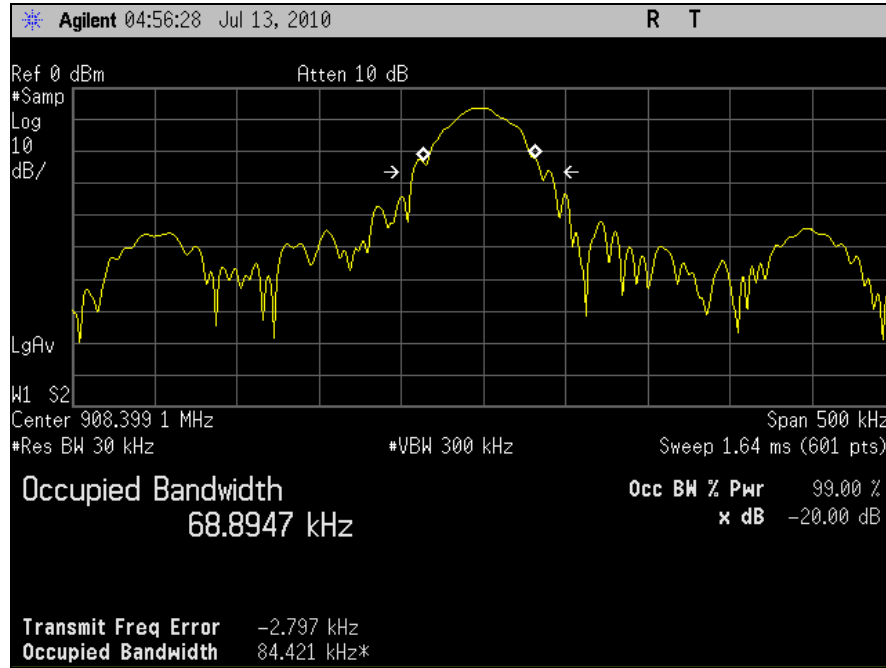
Plot 11. Occupied Bandwidth, IC Limits
