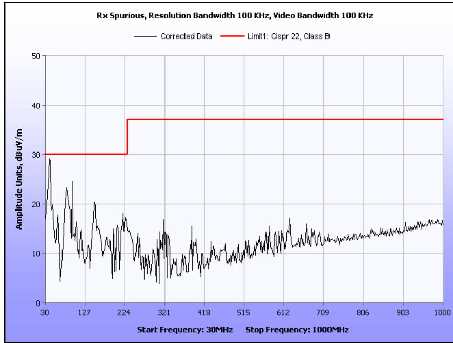
Plot 18. Receiver Spurious Emission, 30 MHz – 1 GHz
