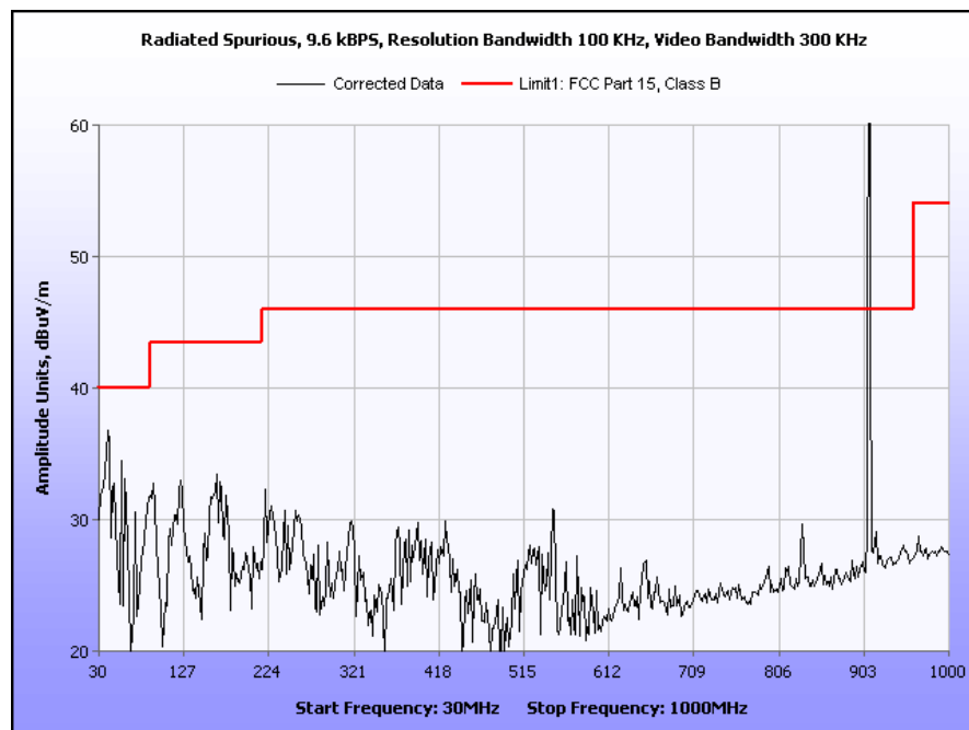
Plot 14. Radiated Spurious Emissions, 9.6 kbps, 30 MHz – 1 GHz
