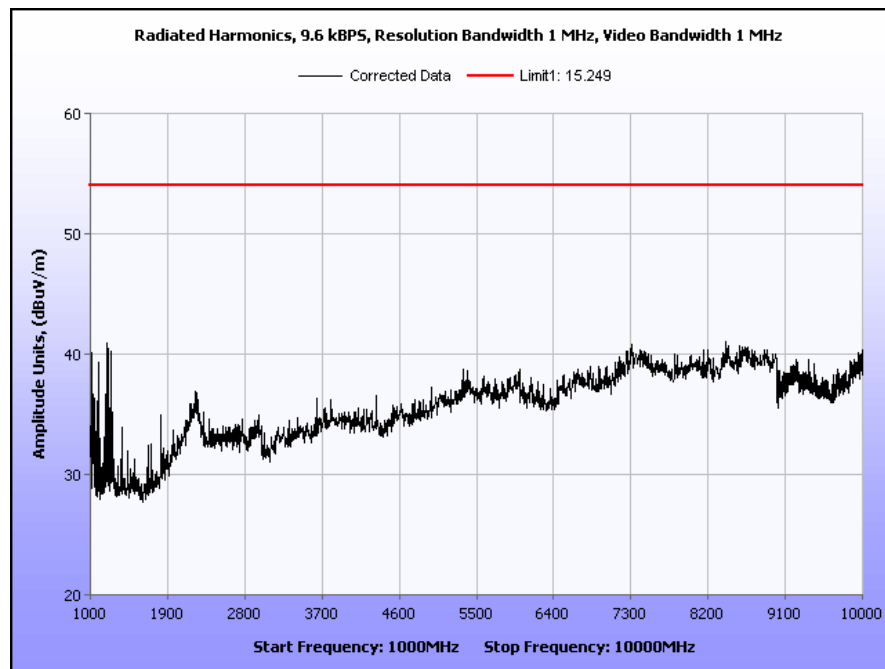
Plot 12. Radiated Harmonics, 9.6kBPS, 1 GHz – 10 GHz
