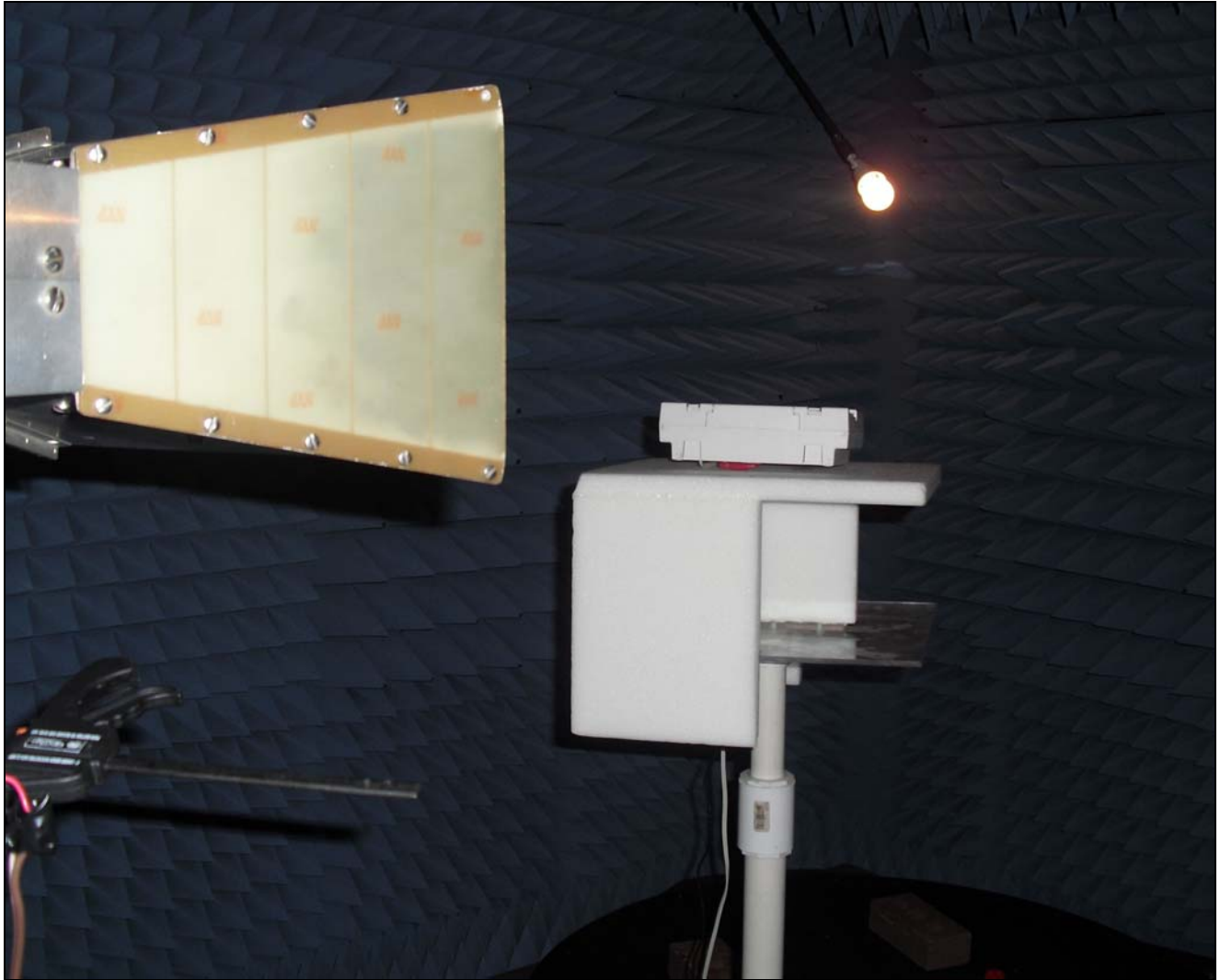
Photograph 7. Host 1, Spurious Transmitter Emissions, Test Setup
