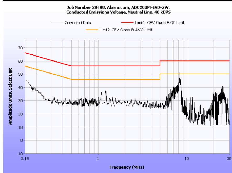
Plot 8. Conducted Emissions, Neutral Line, 40 kBPS
