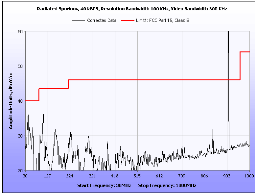
Plot 15. Radiated Spurious Emissions, 40 kbps, 30 MHz – 1 GHz
