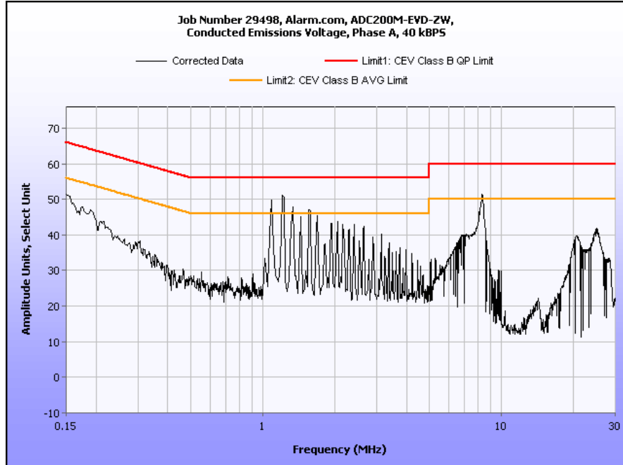
Plot 6. Conducted Emissions, Phase Line, 40 kbps
