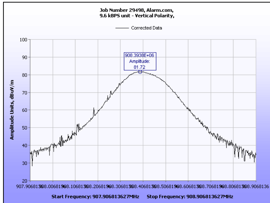
Plot 9. Fundamental Field Strength
