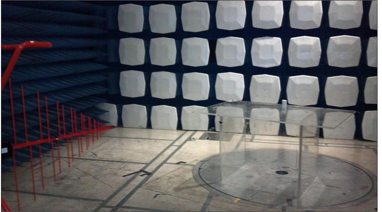
Photograph 4. Radiated Spurious Emissions, Test Setup, Below 1 GHz
