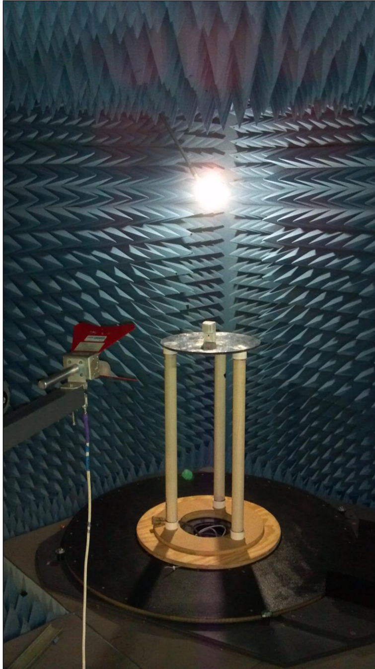
Photograph 2. Radiated Emissions, Test Setup, Above 1 GHz
