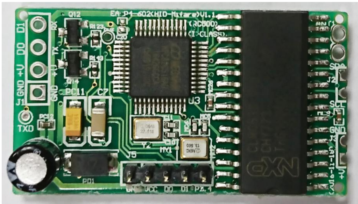
High Frequency PCA – Top View
