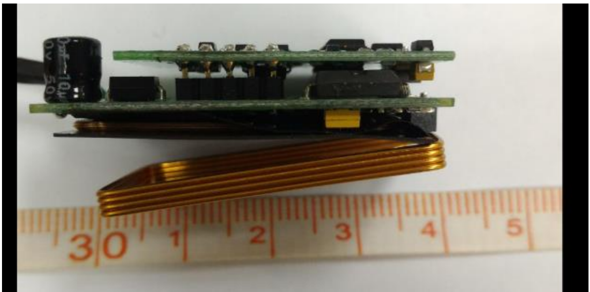
Full Assembly – Side View
