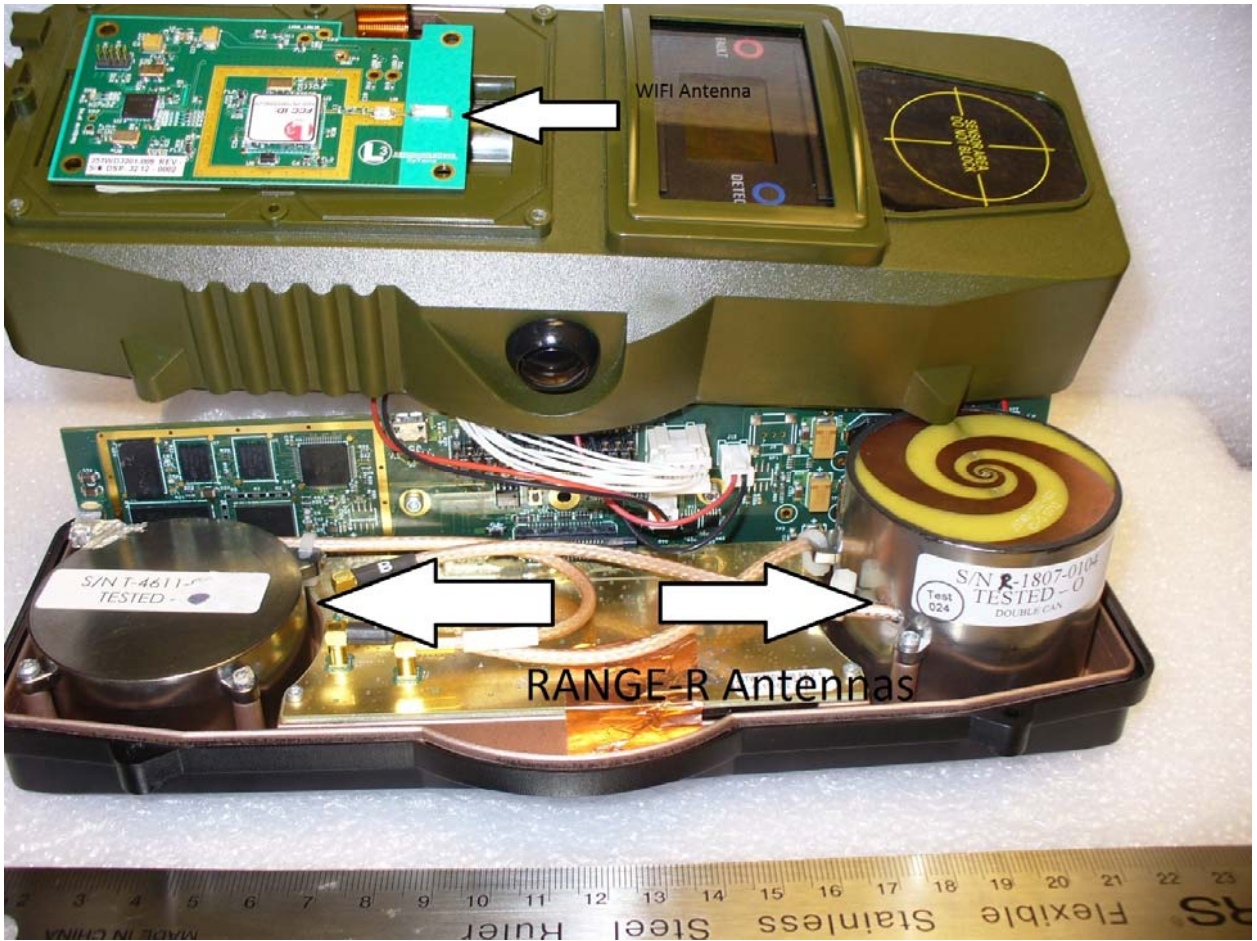
Figure 1: Internal View identifying antenna locations
