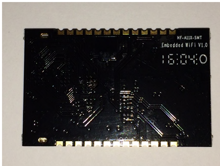
Figure 3: Module – Back
