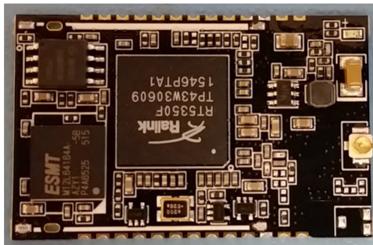
Figure 2: Module – Front without Shields
