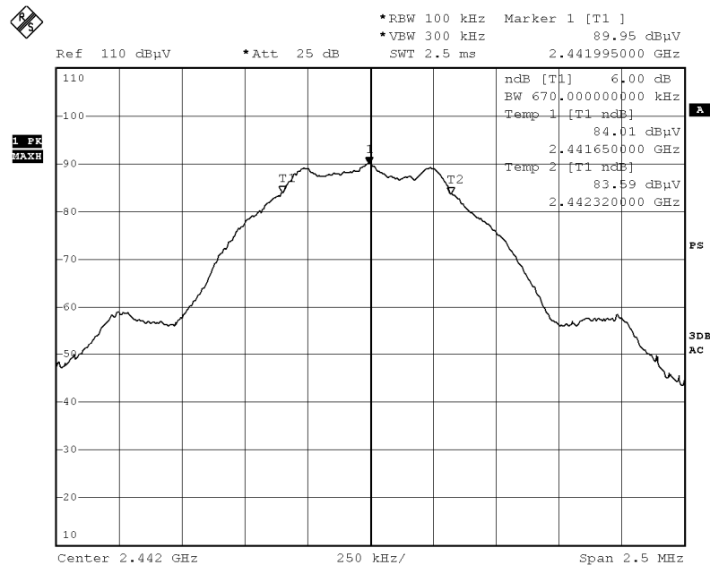
6 dB Bandwidth Plot on Configuration Bluetooth DTS (GFSK: 2442MHz)
