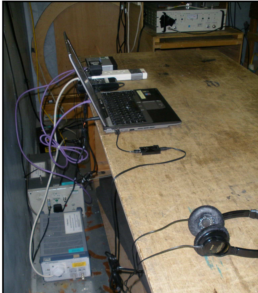
Photograph 2 Conducted Emissions - Back
