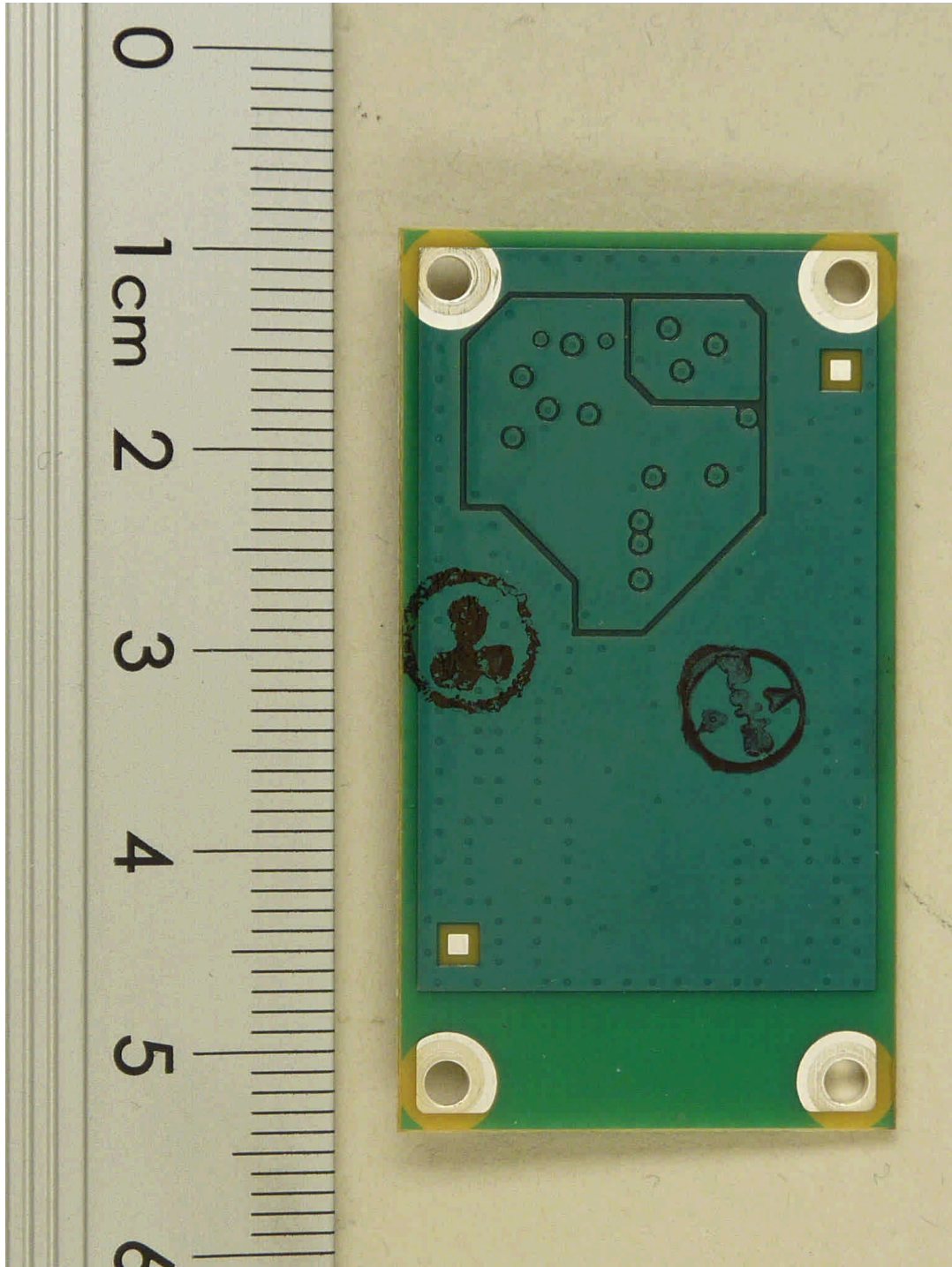
101171_15.jpg Focus Bluetooth Module, PCB, bottom view
