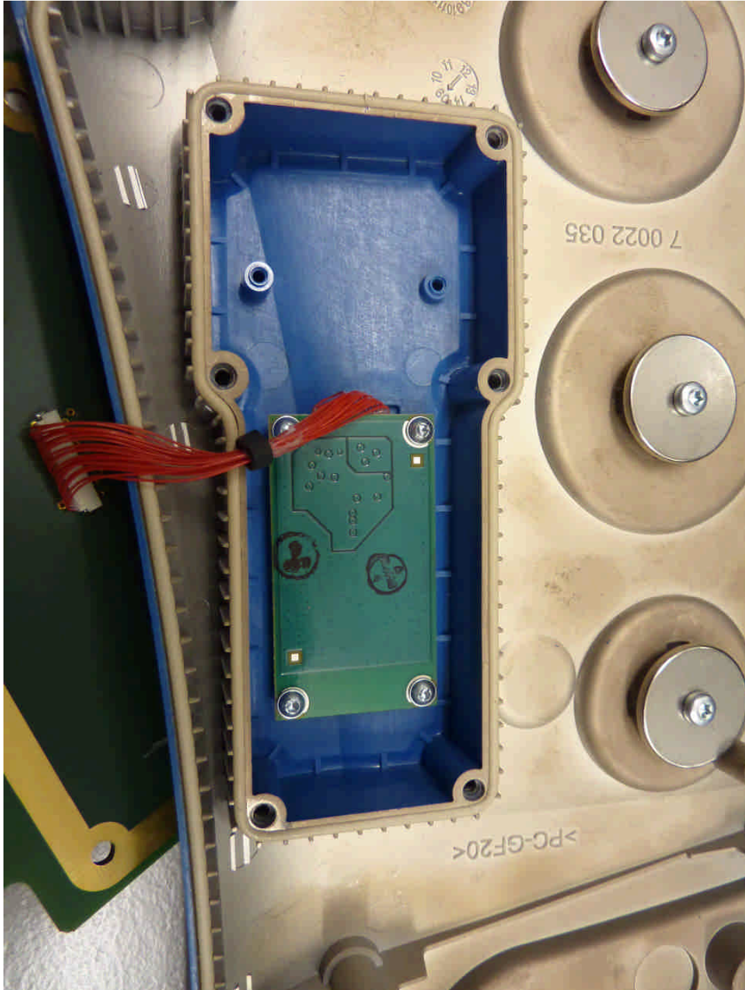
101171_13.jpg FOCUS 30-2", housing of Focus Bluetooth Module PCB
