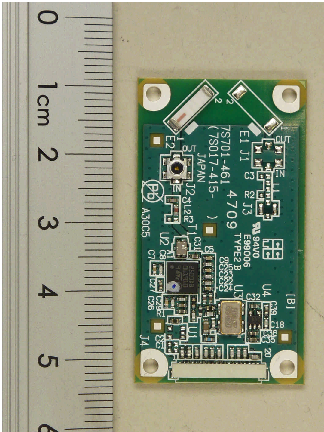
101171_14.jpg Focus Bluetooth Module, PCB, top view
