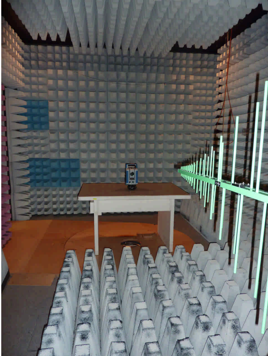
101171_9.jpg FOCUS 30-2“, test set-up fully anechoic chamber
