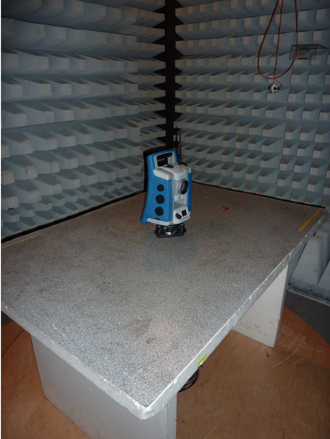
101171_3.jpg FOCUS 30-2“, test set-up fully anechoic chamber
