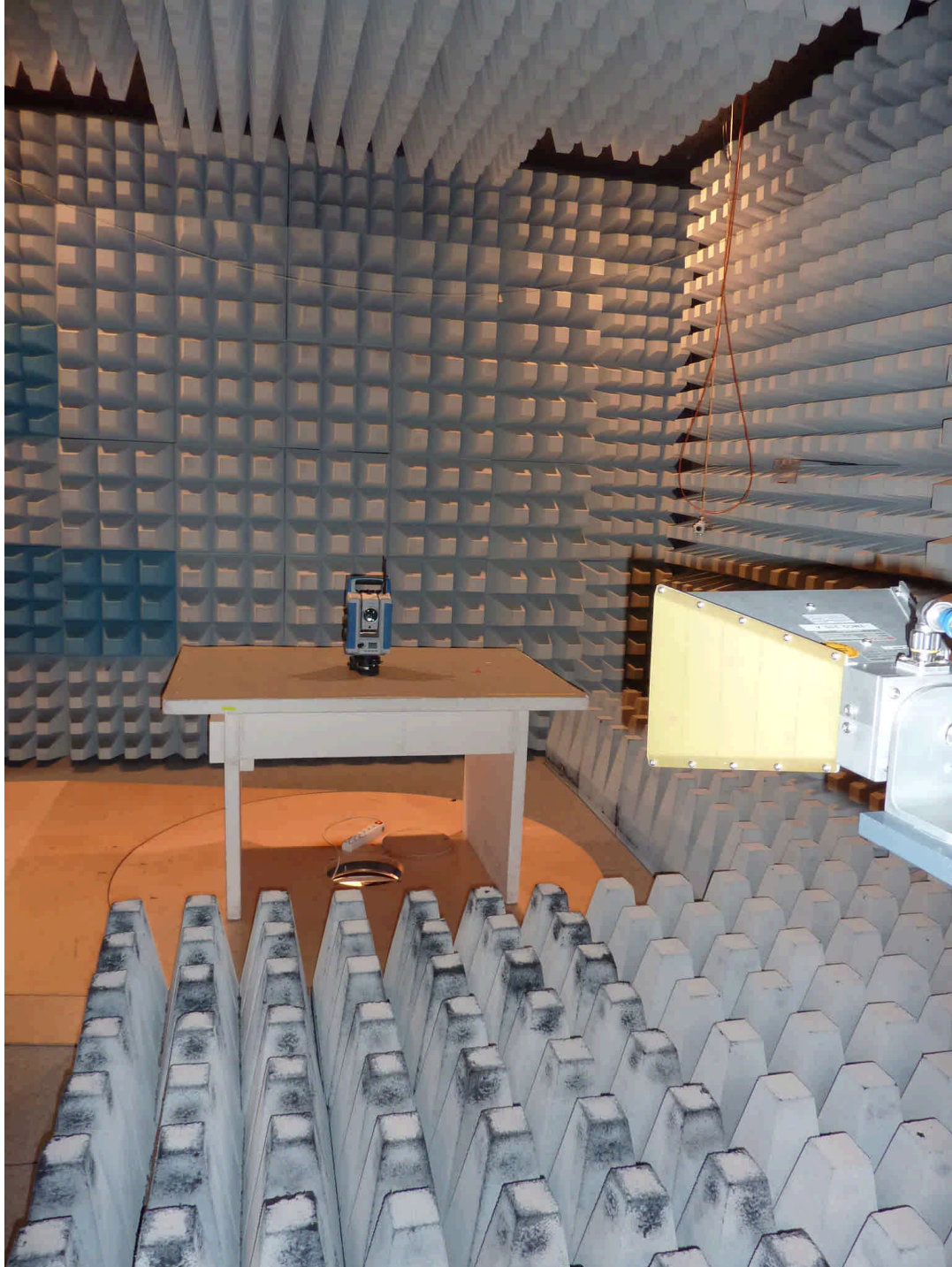
101171_4.jpg FOCUS 30-2“, test set-up fully anechoic chamber
