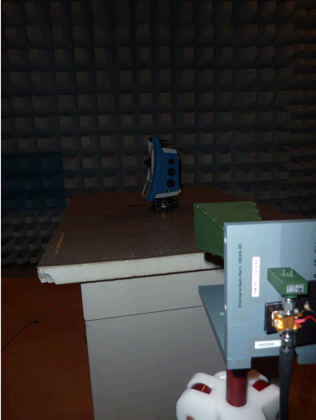
101171_6.jpg FOCUS 30-2“, test set-up fully anechoic chamber
