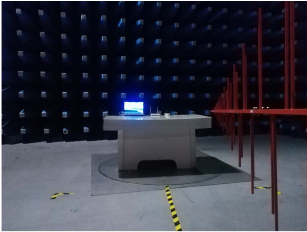
Radiated Emissions Test Setup Below 1GHz - -Adapter: PSAA06A-120
