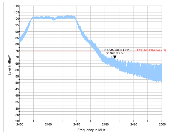
802.11g-Channel 11: Peak
