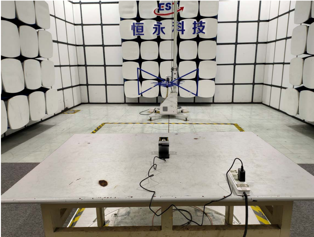
Radiated test: 30M-1GMHz
