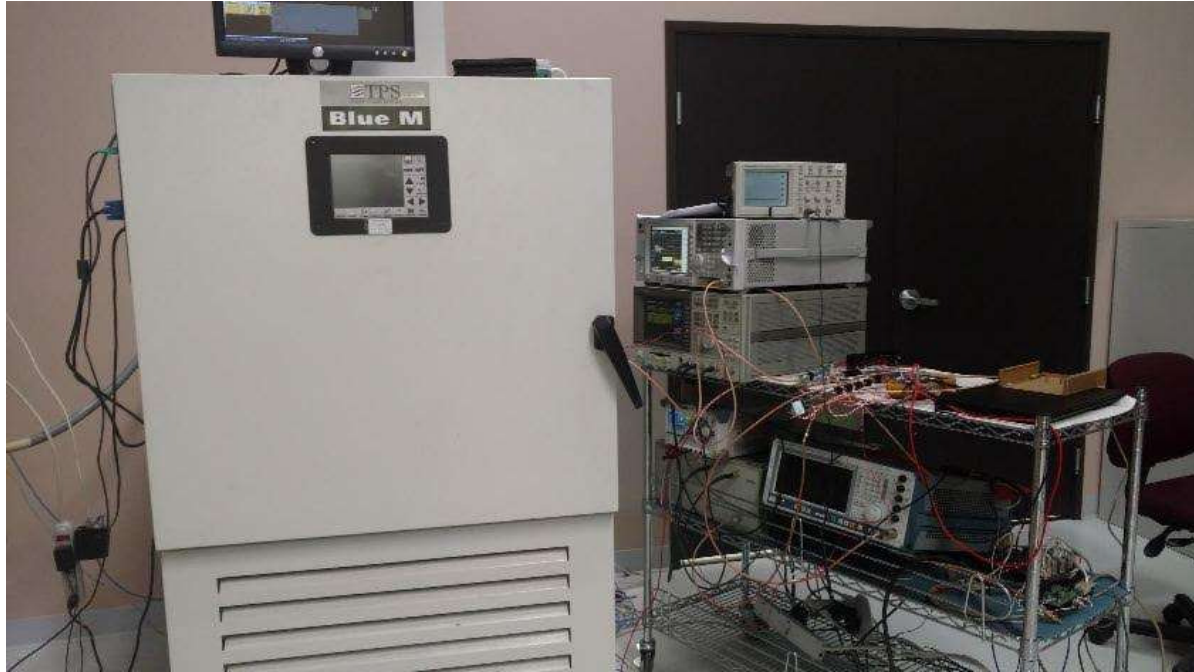
Figure 2: Overall test setup frequency stability
