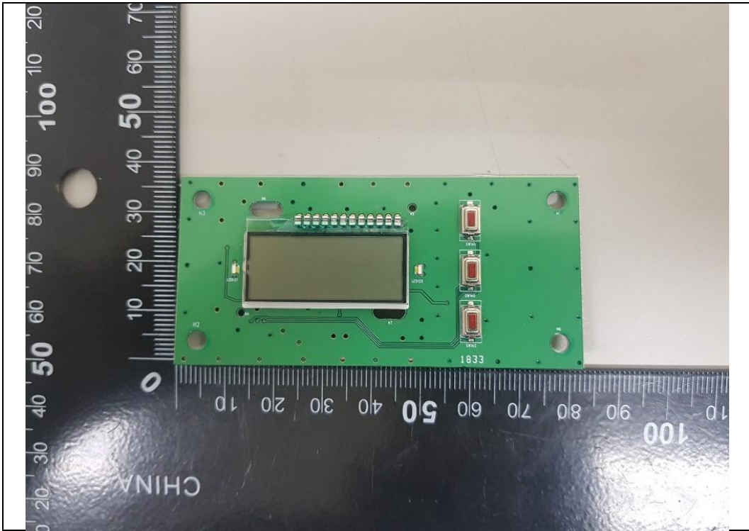
Front LCD&Button_Front
