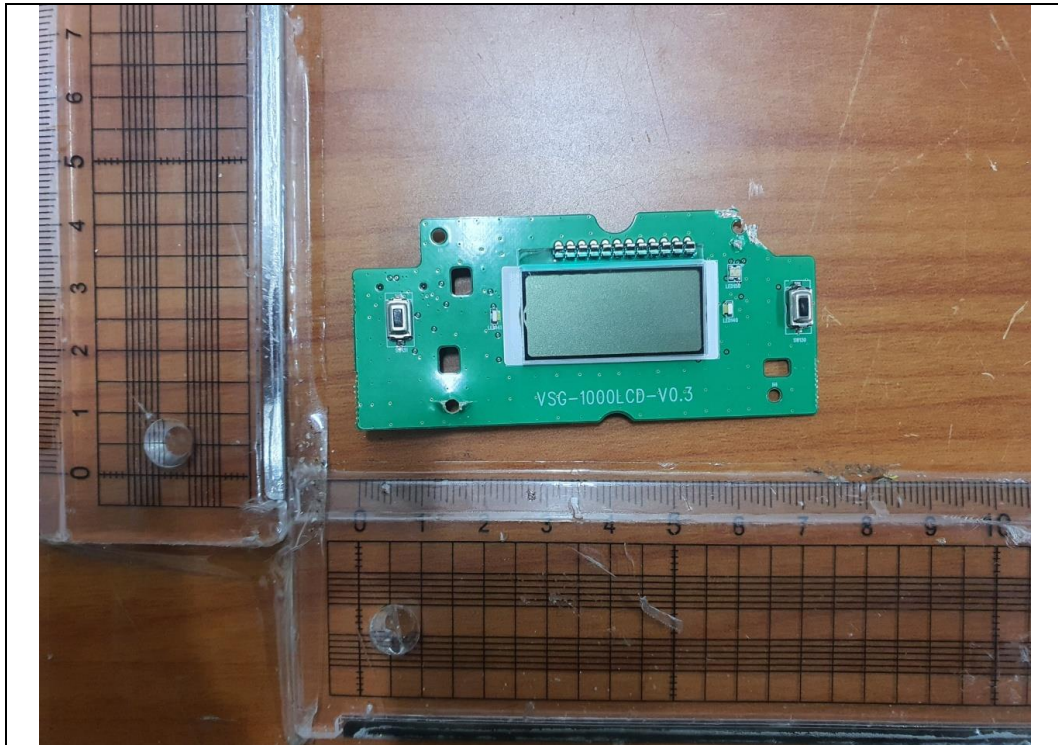
LCD Board Front
